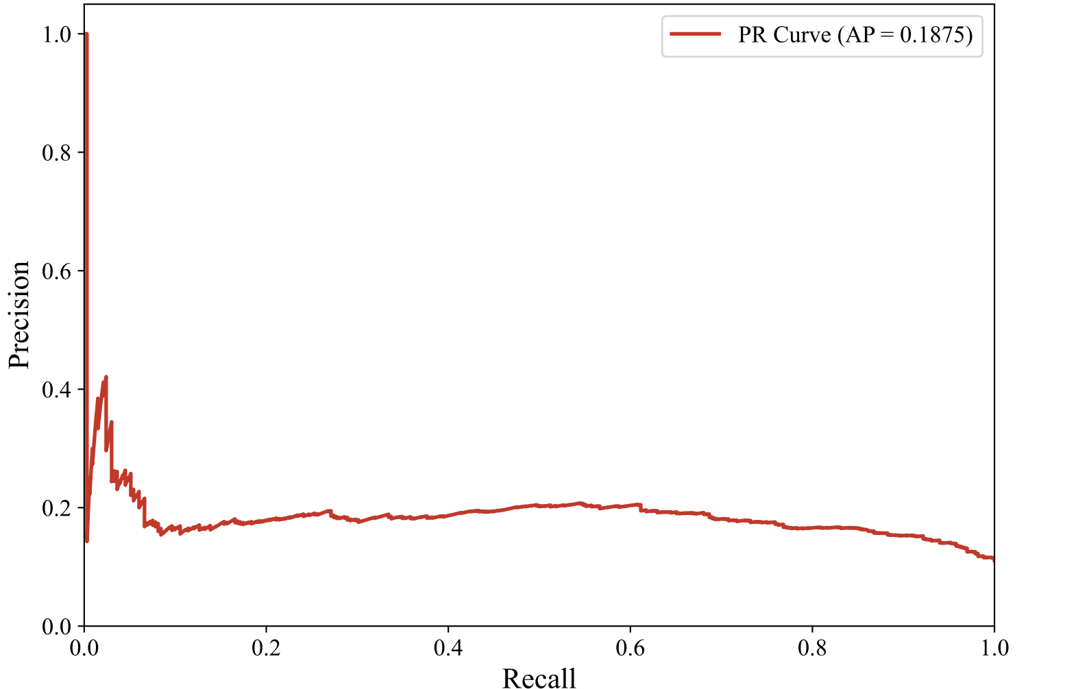
Precision-Recall Curve — GERMAN_MANUAL (paraphrase-multilingual-mpnet-base-v2, svm_rbf)
