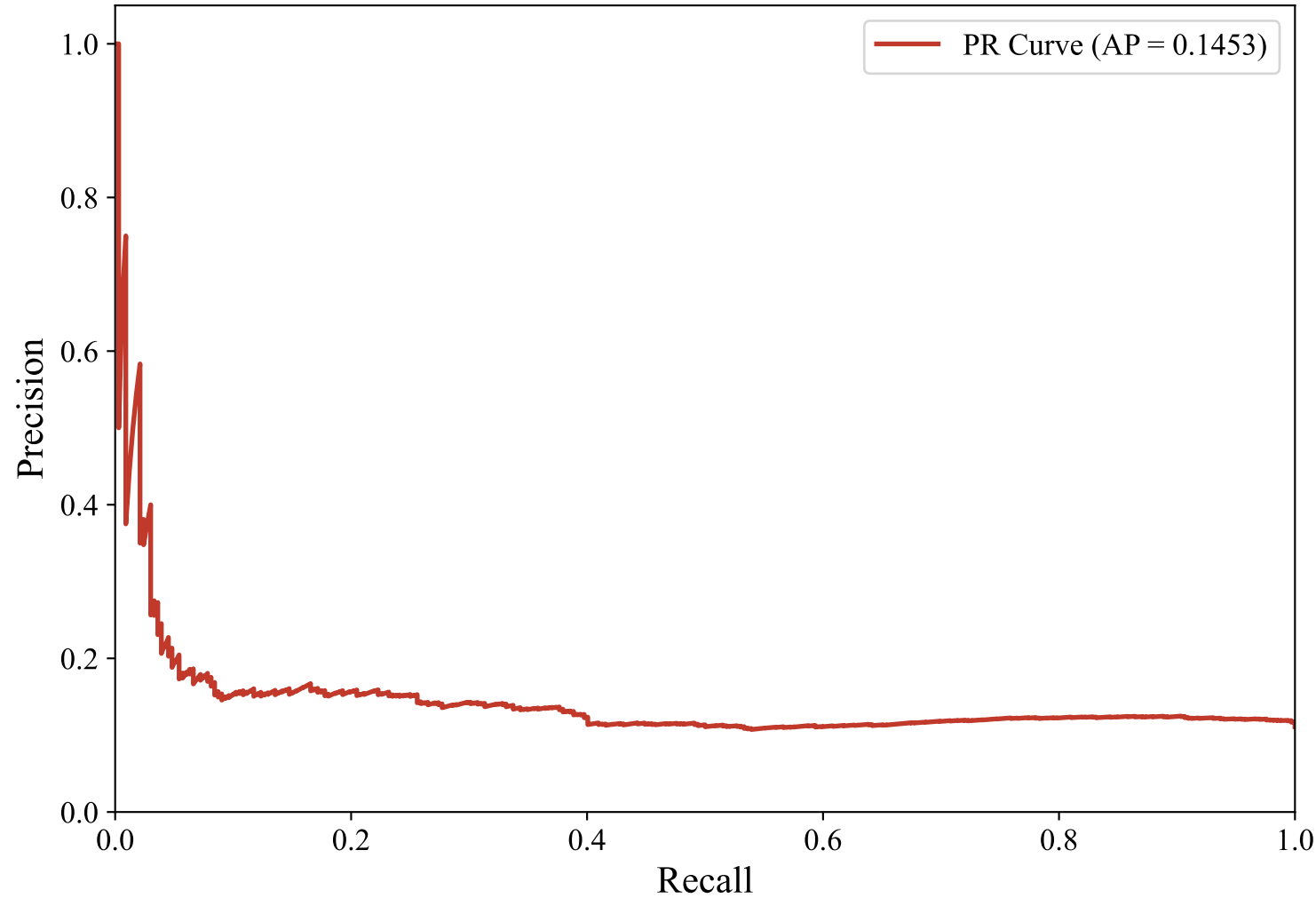
Precision-Recall Curve — GERMAN_MANUAL (snowflake-arctic-embed-l-v2.0, lightgbm)
