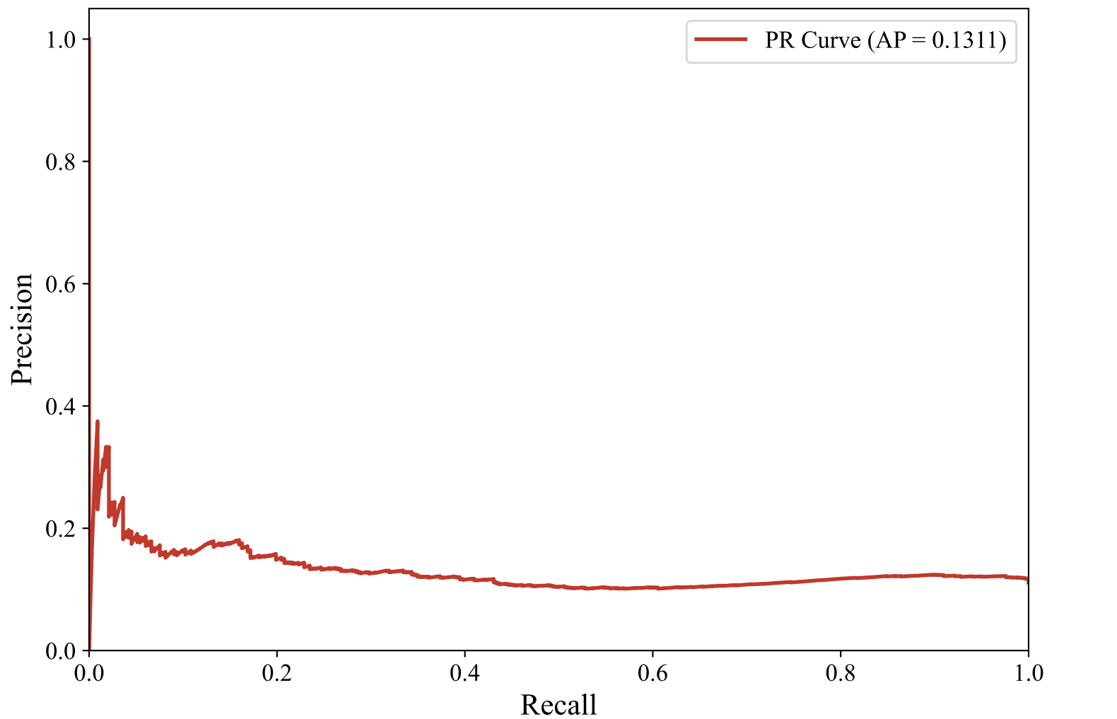
Precision-Recall Curve — GERMAN_MANUAL (xlm-roberta-base, lightgbm)
