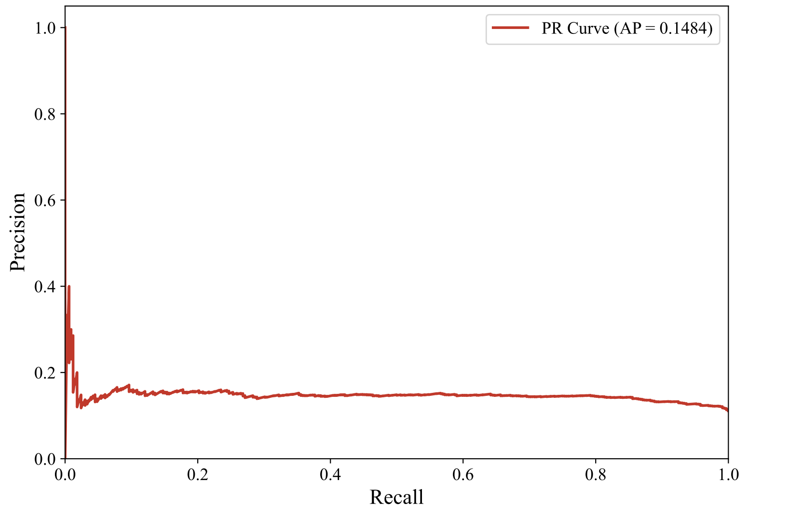
Precision-Recall Curve — GERMAN_MANUAL (xlm-roberta-base, random_forest)
