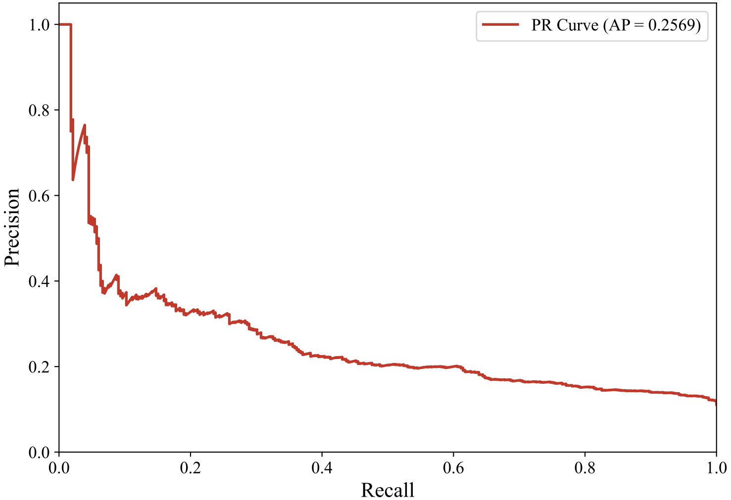
Precision-Recall Curve — GERMAN_MANUAL (xlm-roberta-base, svm_rbf)
