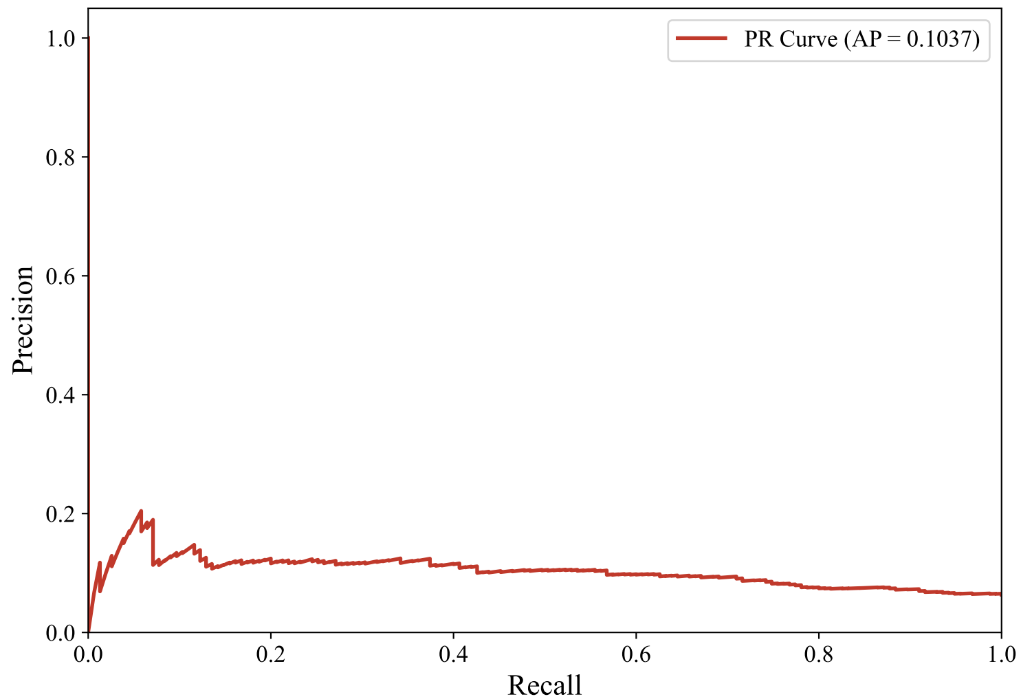
Precision-Recall Curve — SWEDISH_MANUAL (bert-base-multilingual-uncased, svm_linear)
