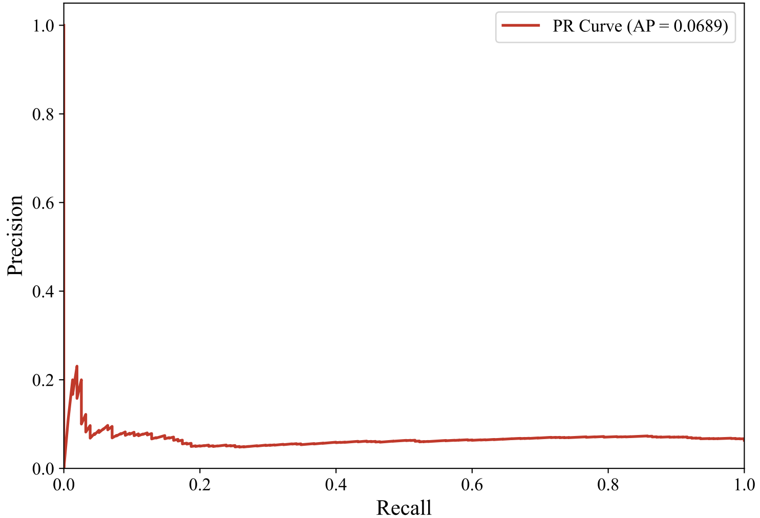
Precision-Recall Curve — SWEDISH_MANUAL (multilingual-e5-large-instruct, xgboost)
