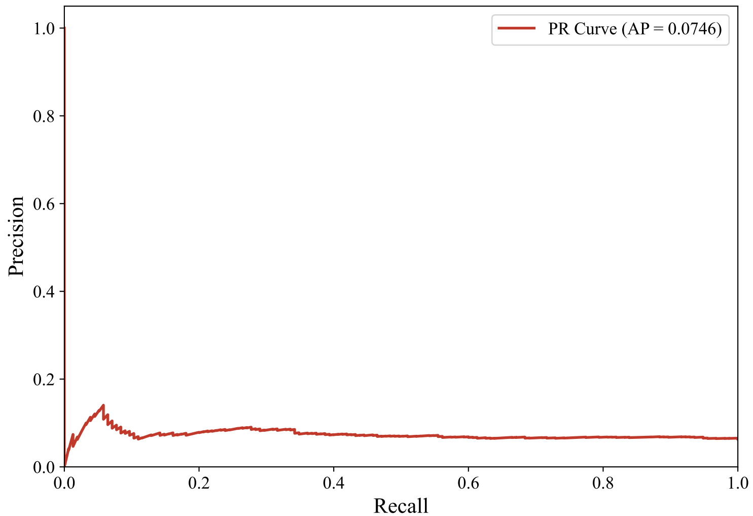
Precision-Recall Curve — SWEDISH_MANUAL (paraphrase-multilingual-MiniLM-L12-v2, svm_rbf)
