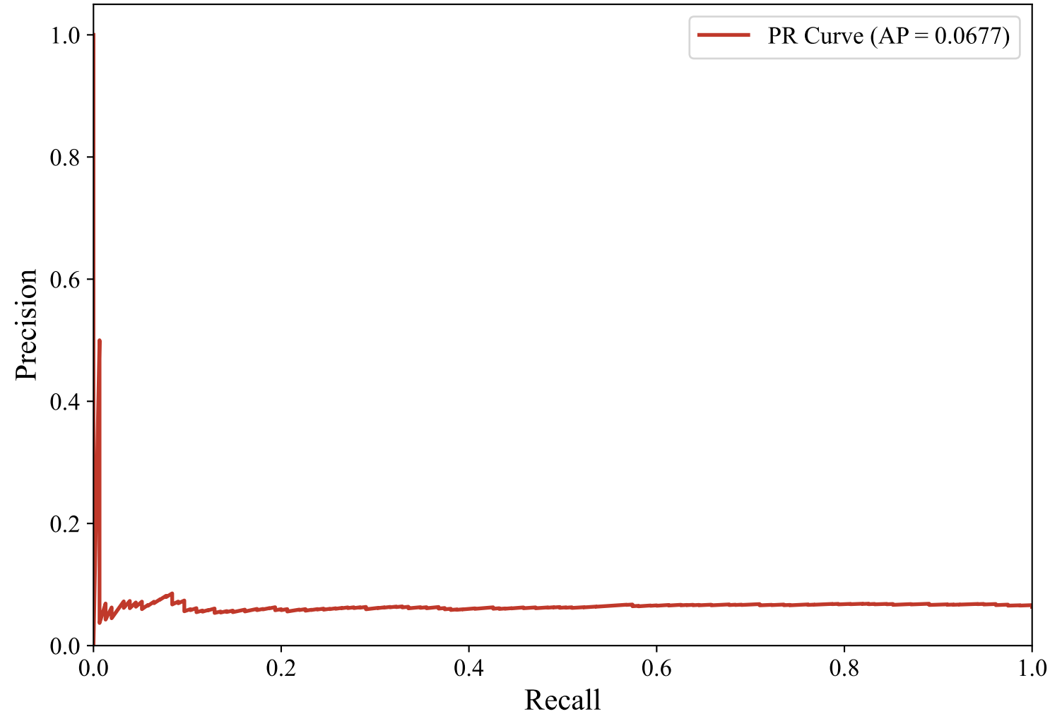
Precision-Recall Curve — SWEDISH_MANUAL (paraphrase-multilingual-MiniLM-L12-v2, xgboost)
