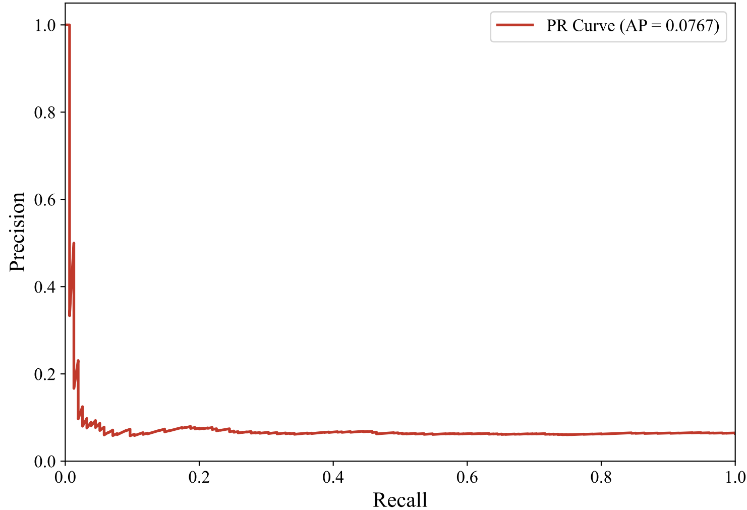
Precision-Recall Curve — SWEDISH_MANUAL (paraphrase-multilingual-mpnet-base-v2, lightgbm)
