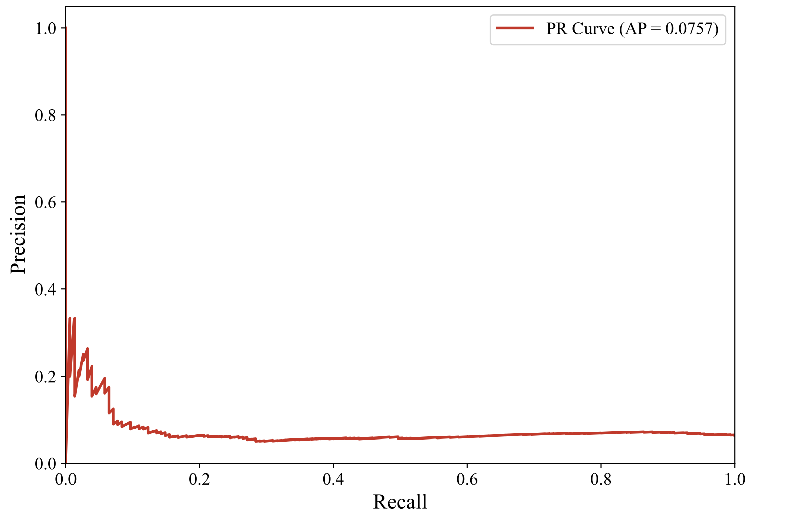
Precision-Recall Curve — SWEDISH_MANUAL (snowflake-arctic-embed-l-v2.0, random_forest)
