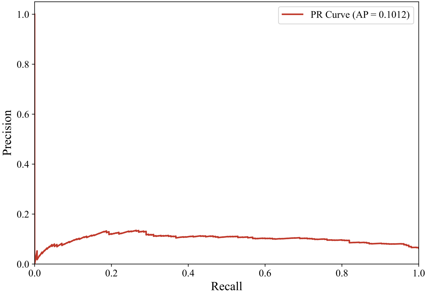
Precision-Recall Curve — SWEDISH_MANUAL (snowflake-arctic-embed-l-v2.0, svm_linear)
