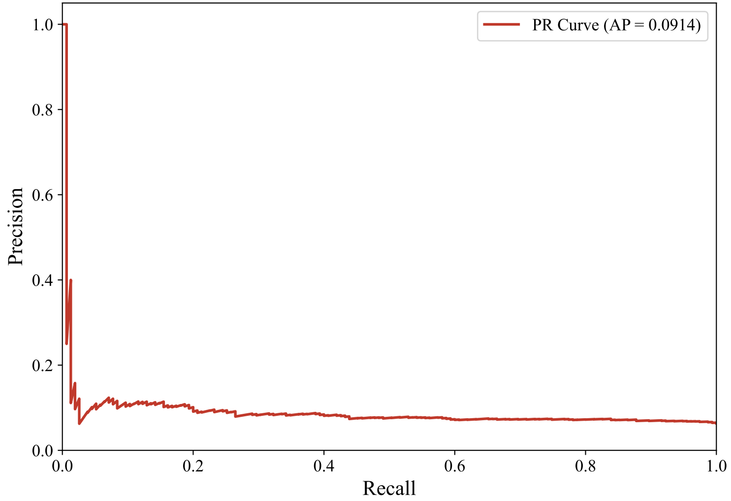
Precision-Recall Curve — SWEDISH_MANUAL (snowflake-arctic-embed-l-v2.0, svm_rbf)
