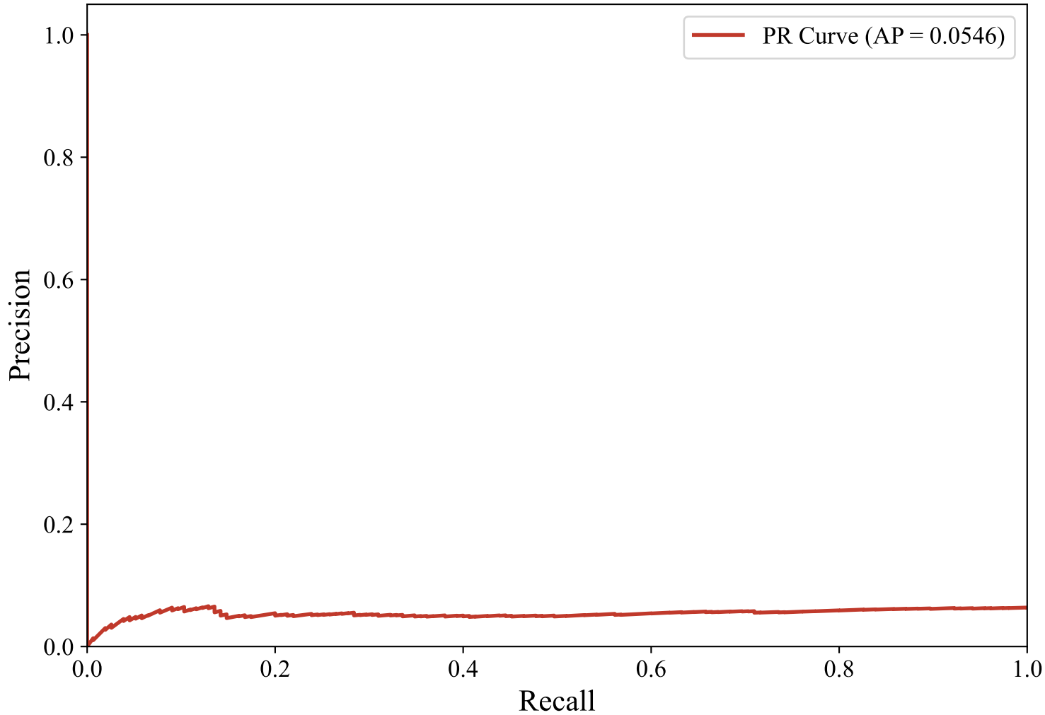
Precision-Recall Curve — SWEDISH_MANUAL (xlm-roberta-base, random_forest)
