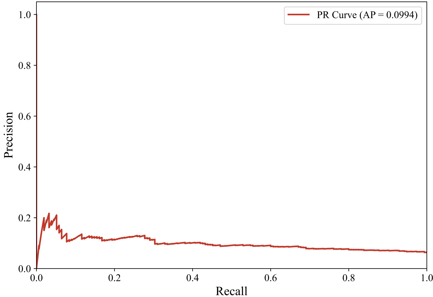
Precision-Recall Curve — SWEDISH_MANUAL (xlm-roberta-base, svm_linear)
