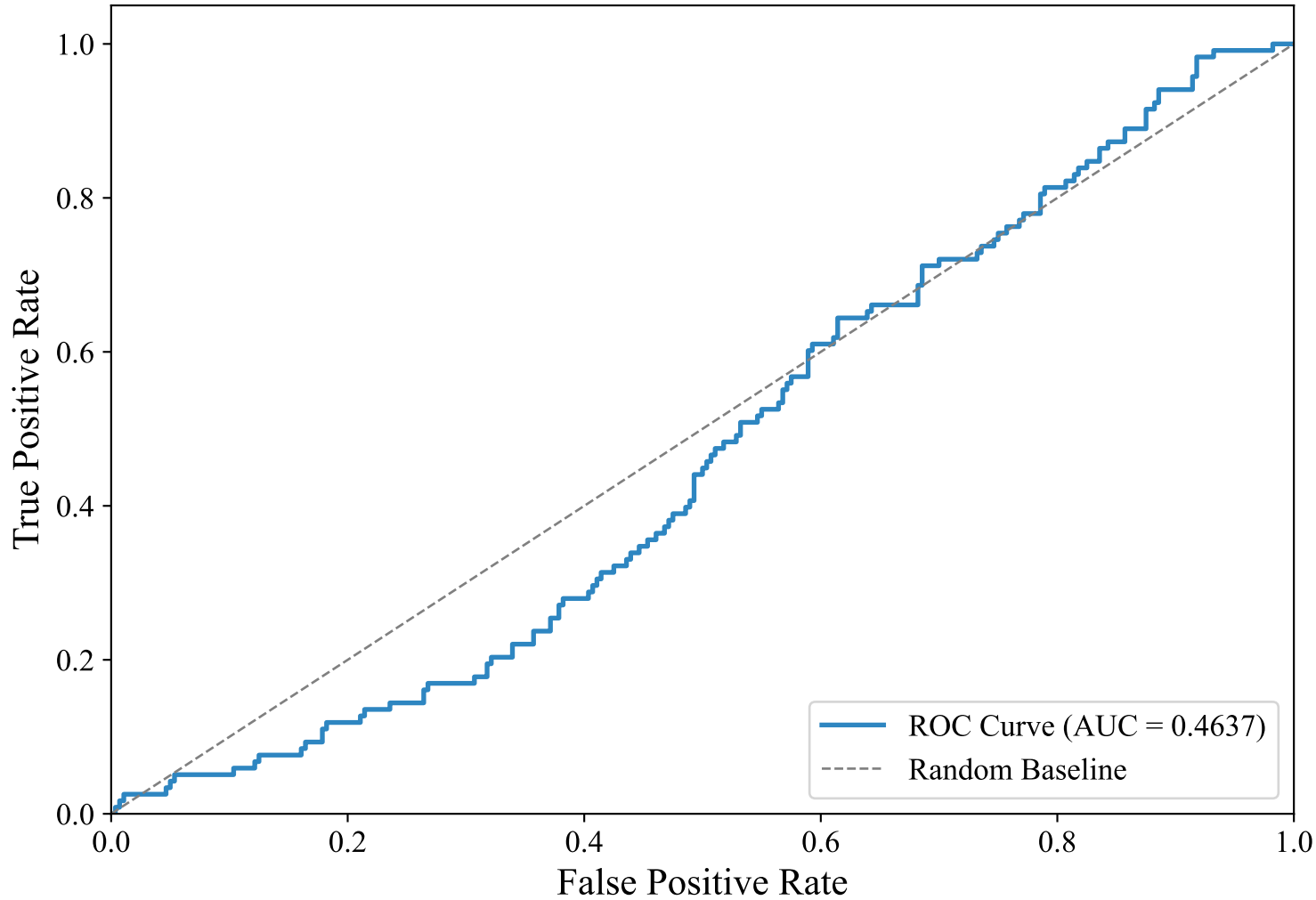
ROC Curve — DUTCH_MANUAL (bert-base-multilingual-uncased, lightgbm)
