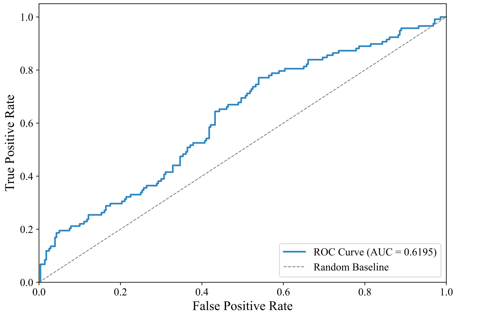
ROC Curve — DUTCH_MANUAL (bert-base-multilingual-uncased, svm_rbf)
