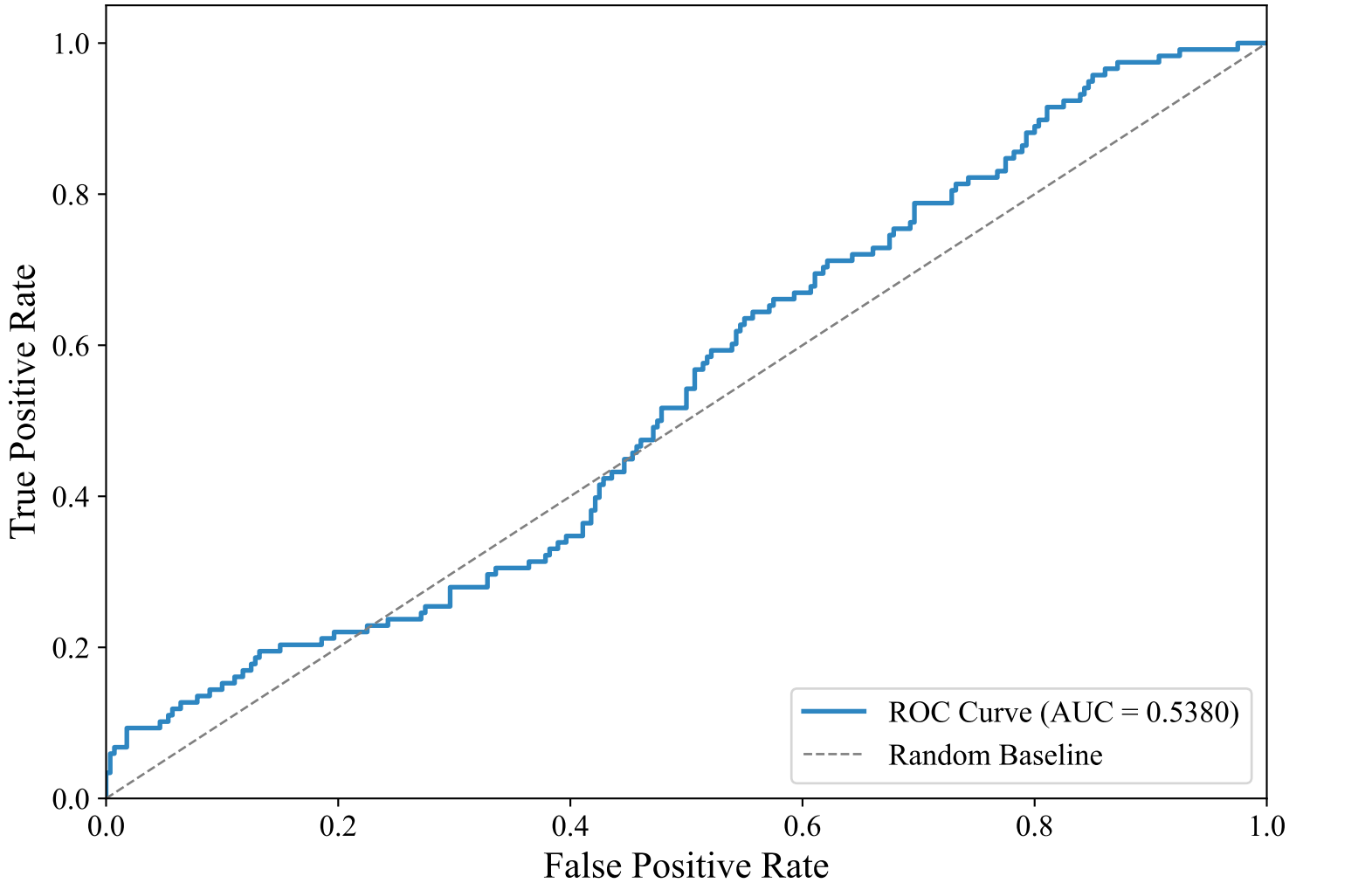
ROC Curve — DUTCH_MANUAL (multilingual-e5-large-instruct, xgboost)
