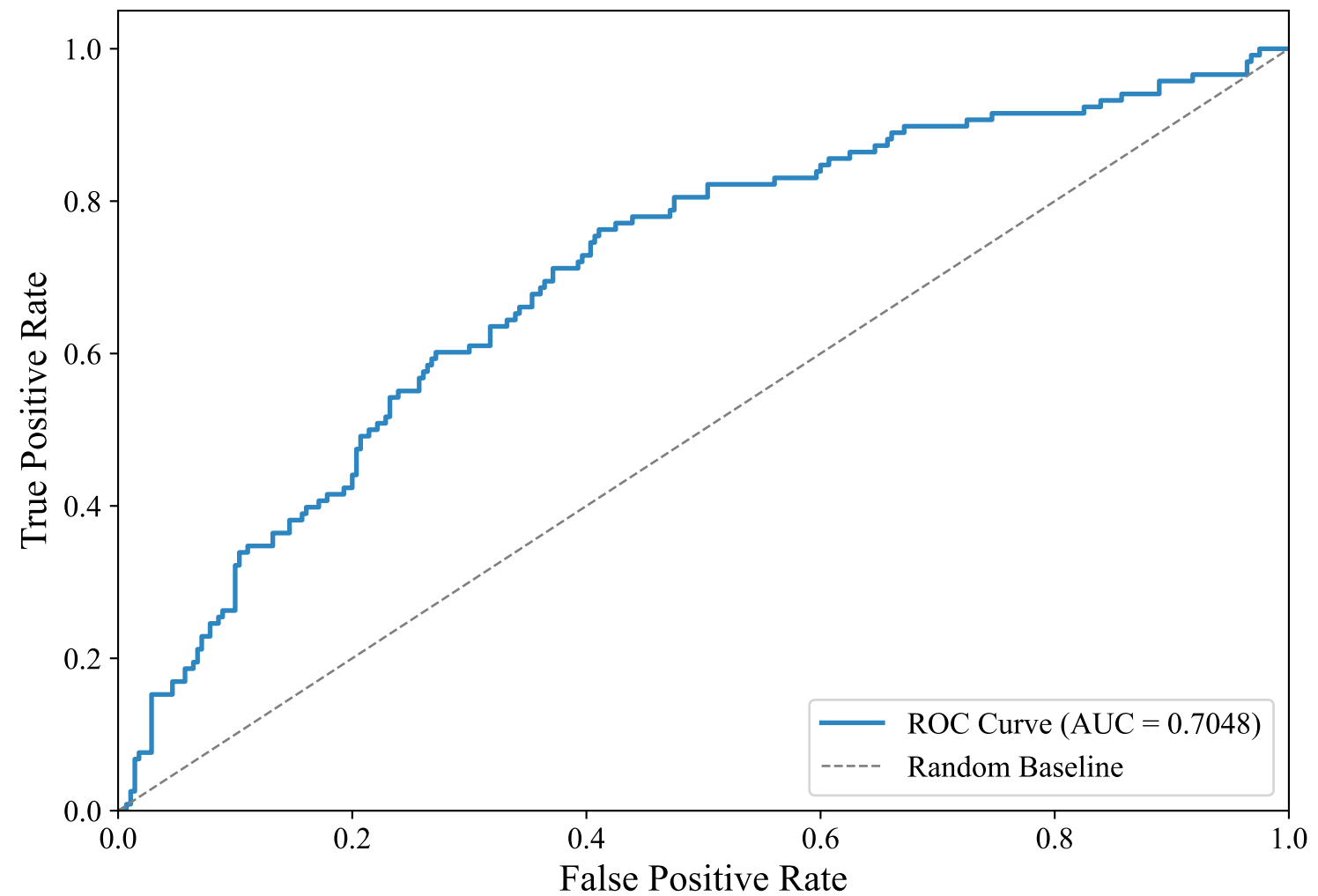
ROC Curve — DUTCH_MANUAL (paraphrase-multilingual-MiniLM-L12-v2, random_forest)
