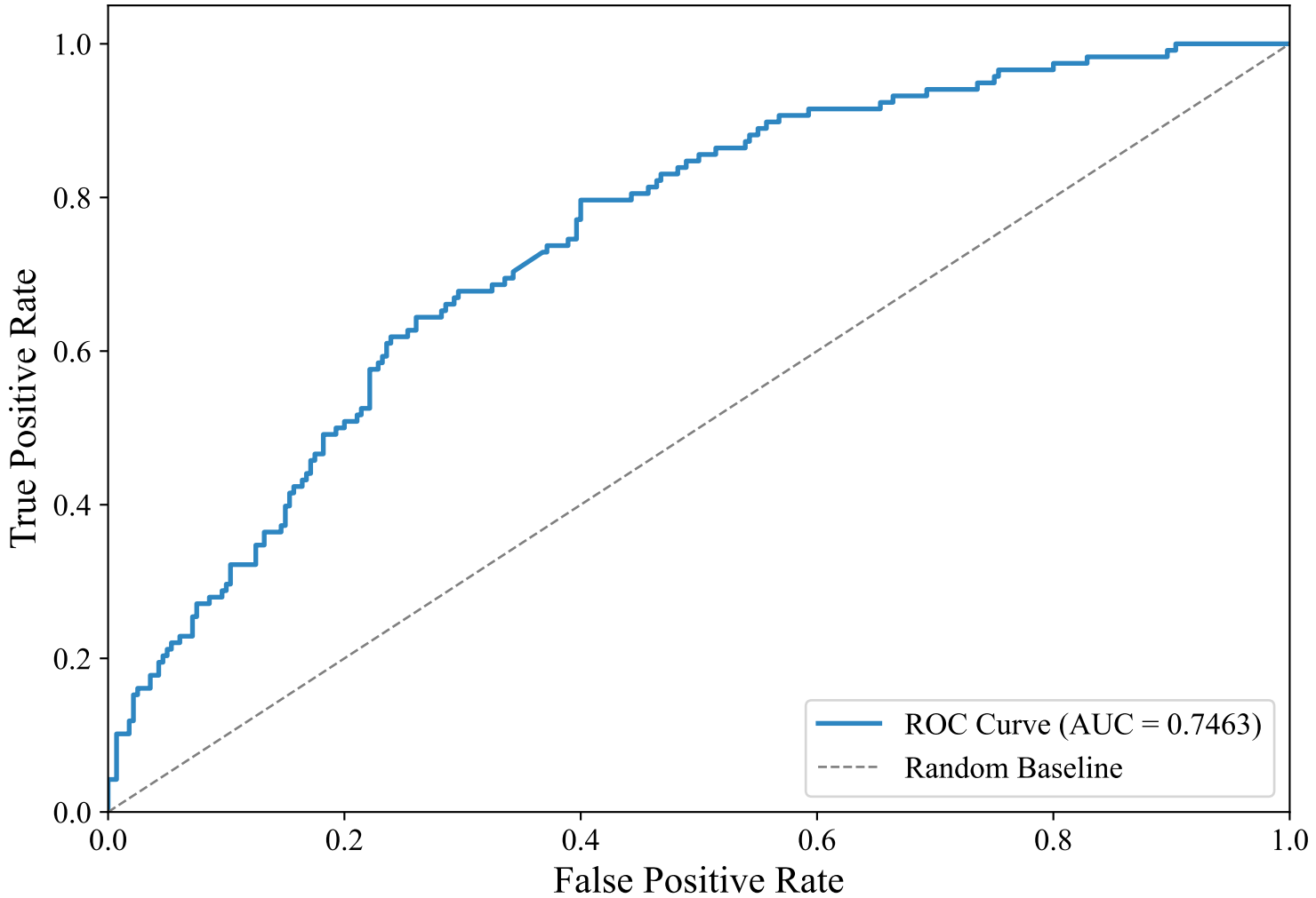
ROC Curve — DUTCH_MANUAL (paraphrase-multilingual-mpnet-base-v2, svm_rbf)
