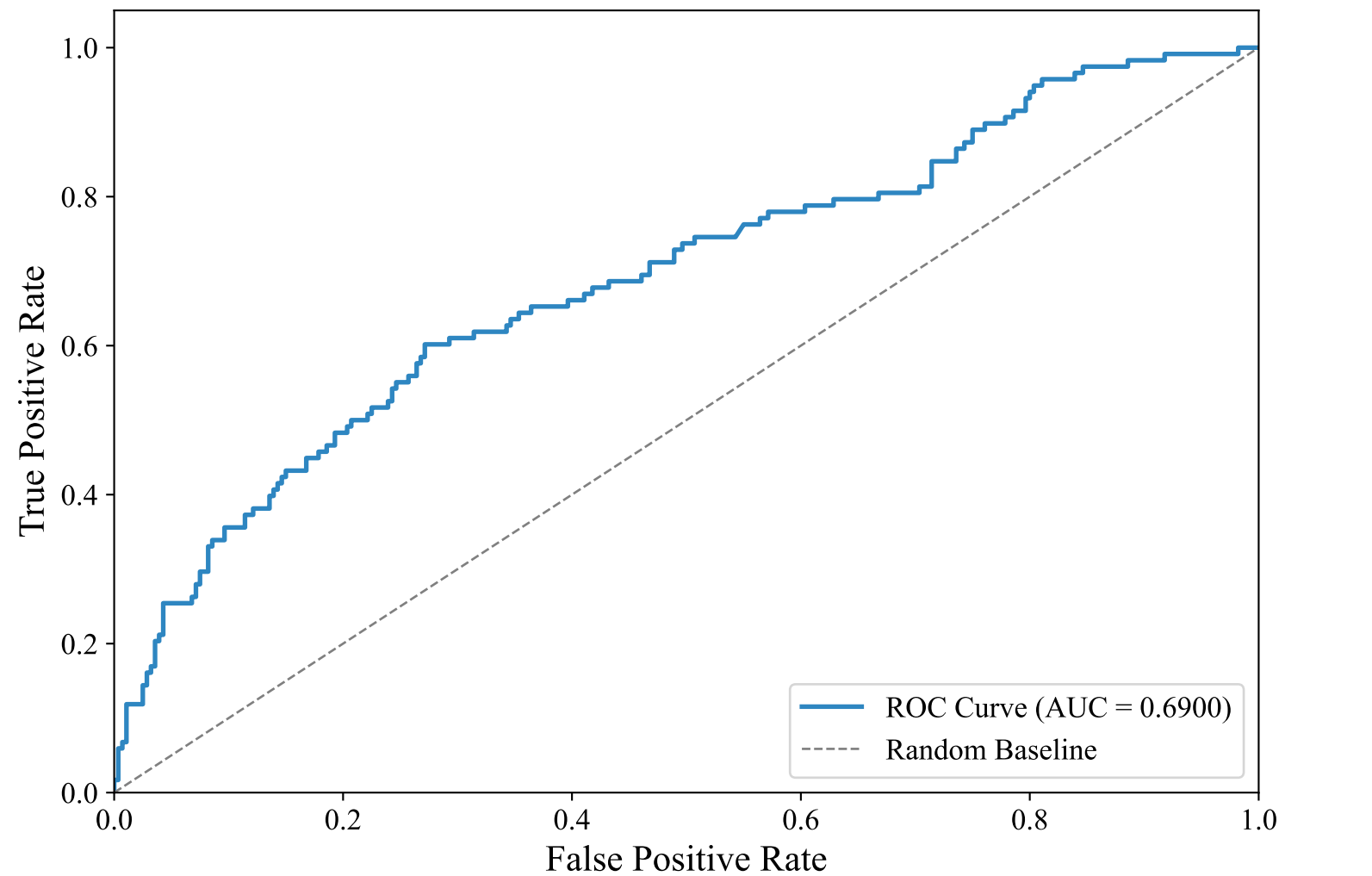
ROC Curve — DUTCH_MANUAL (snowflake-arctic-embed-l-v2.0, svm_rbf)
