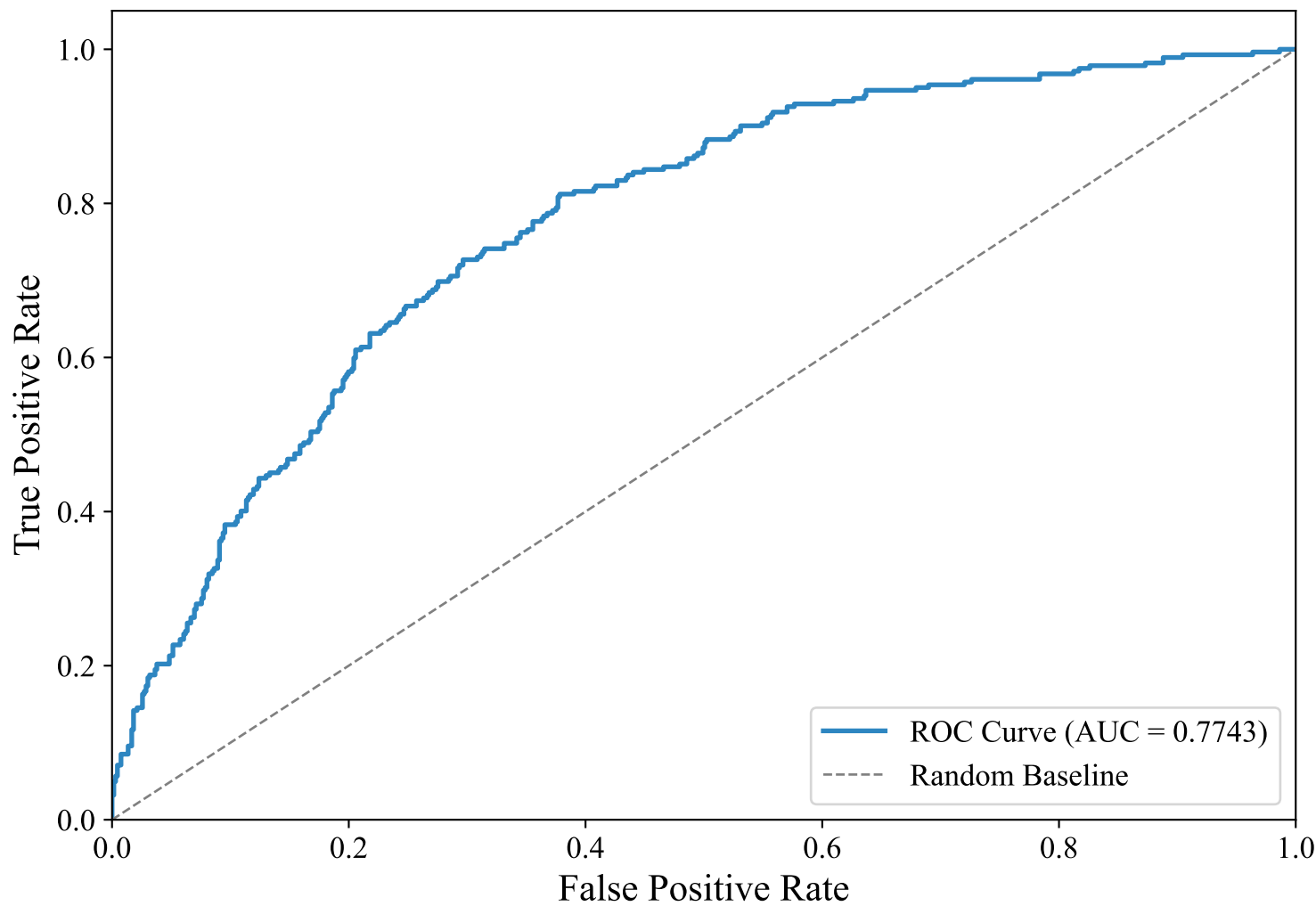
ROC Curve — ENGLISH_MANUAL (multilingual-e5-large-instruct, svm_linear)
