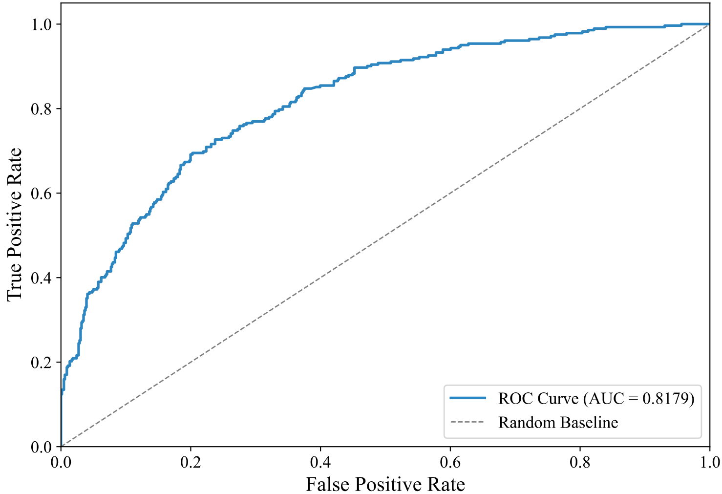
ROC Curve — ENGLISH_MANUAL (multilingual-e5-large-instruct, svm_rbf)
