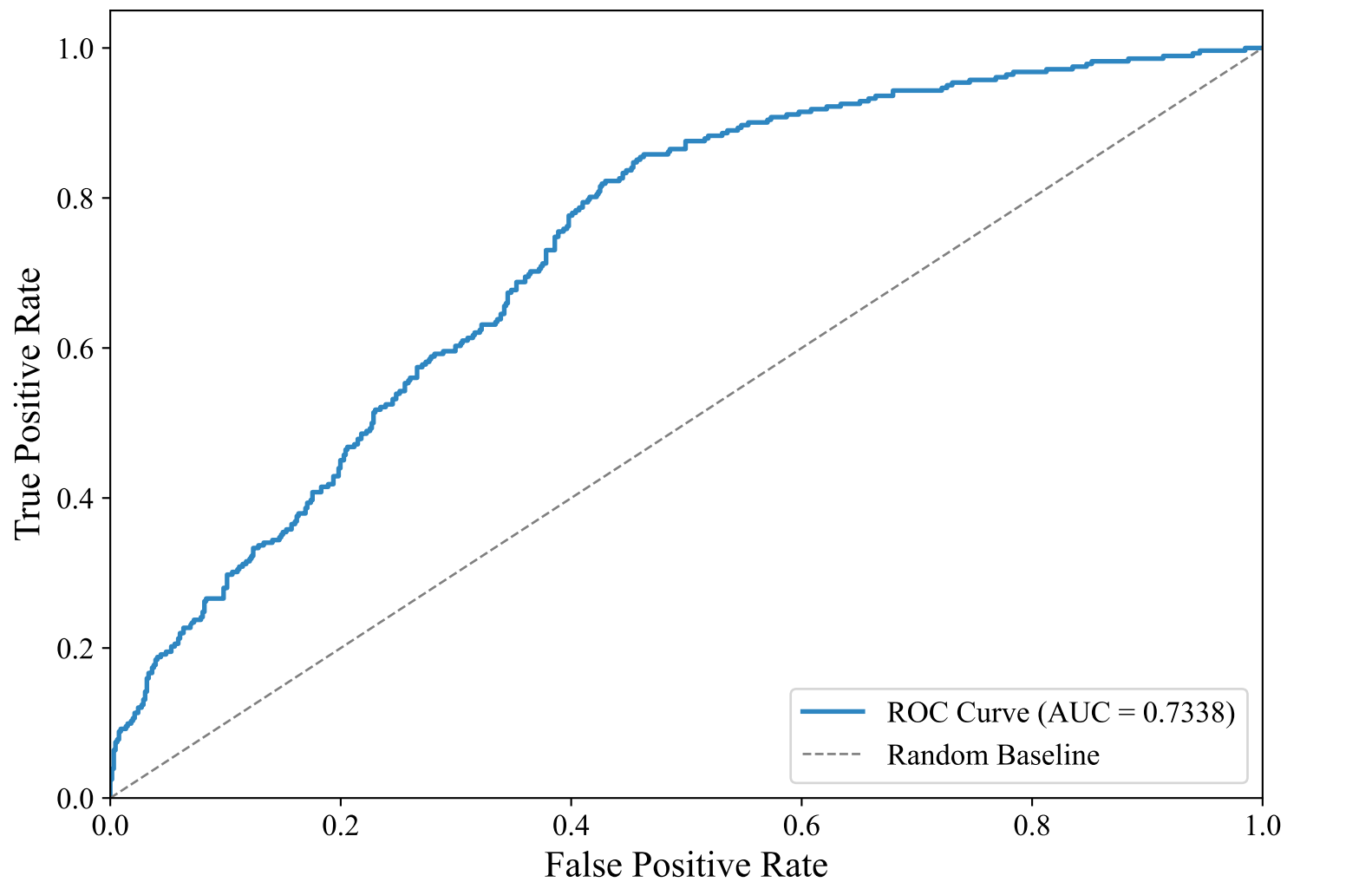
ROC Curve — ENGLISH_MANUAL (multilingual-e5-large-instruct, xgboost)
