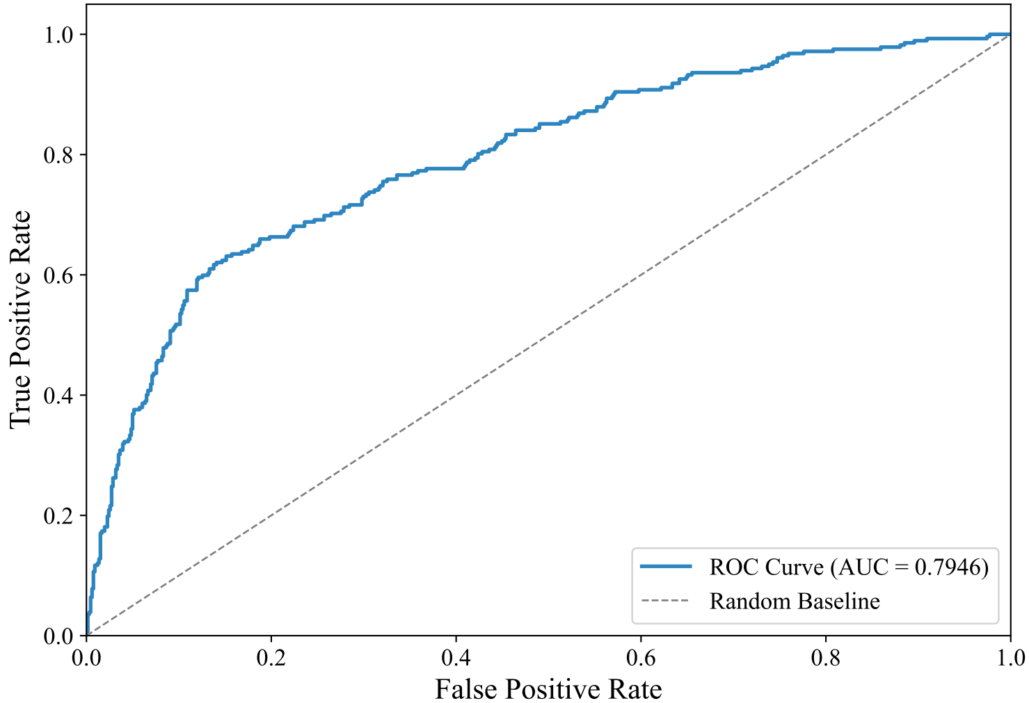
ROC Curve — ENGLISH_MANUAL (paraphrase-multilingual-MiniLM-L12-v2, lightgbm)
