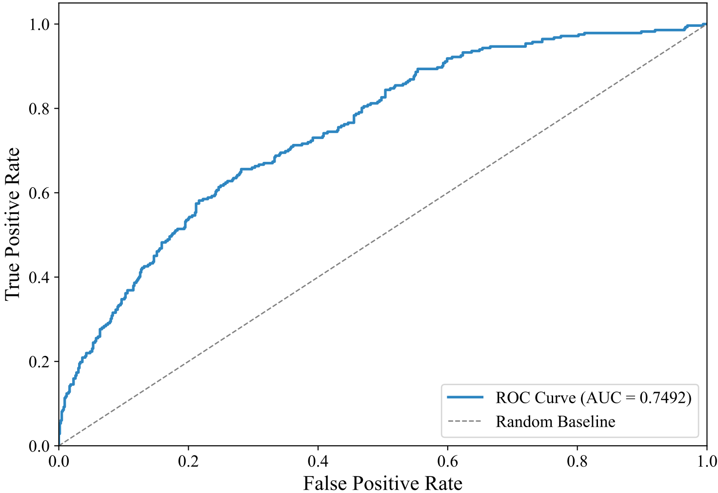
ROC Curve — ENGLISH_MANUAL (paraphrase-multilingual-MiniLM-L12-v2, svm_linear)
