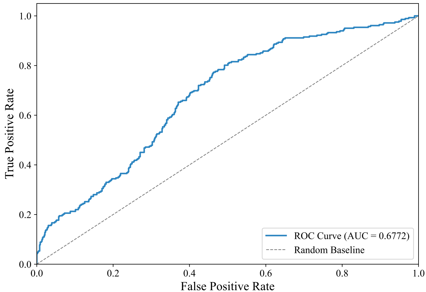
ROC Curve — ENGLISH_MANUAL (snowflake-arctic-embed-l-v2.0, lightgbm)
