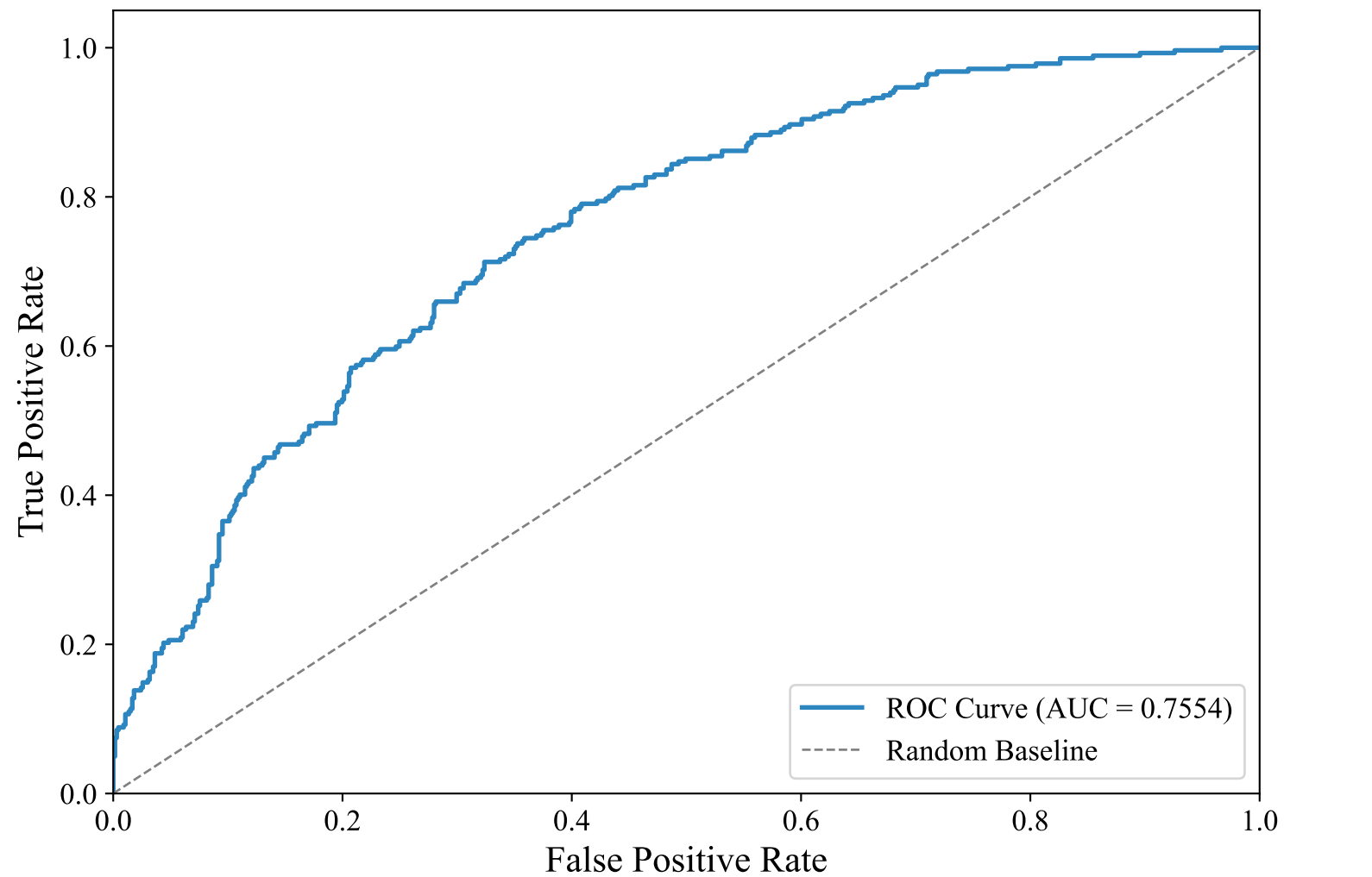
ROC Curve — ENGLISH_MANUAL (snowflake-arctic-embed-l-v2.0, svm_linear)
