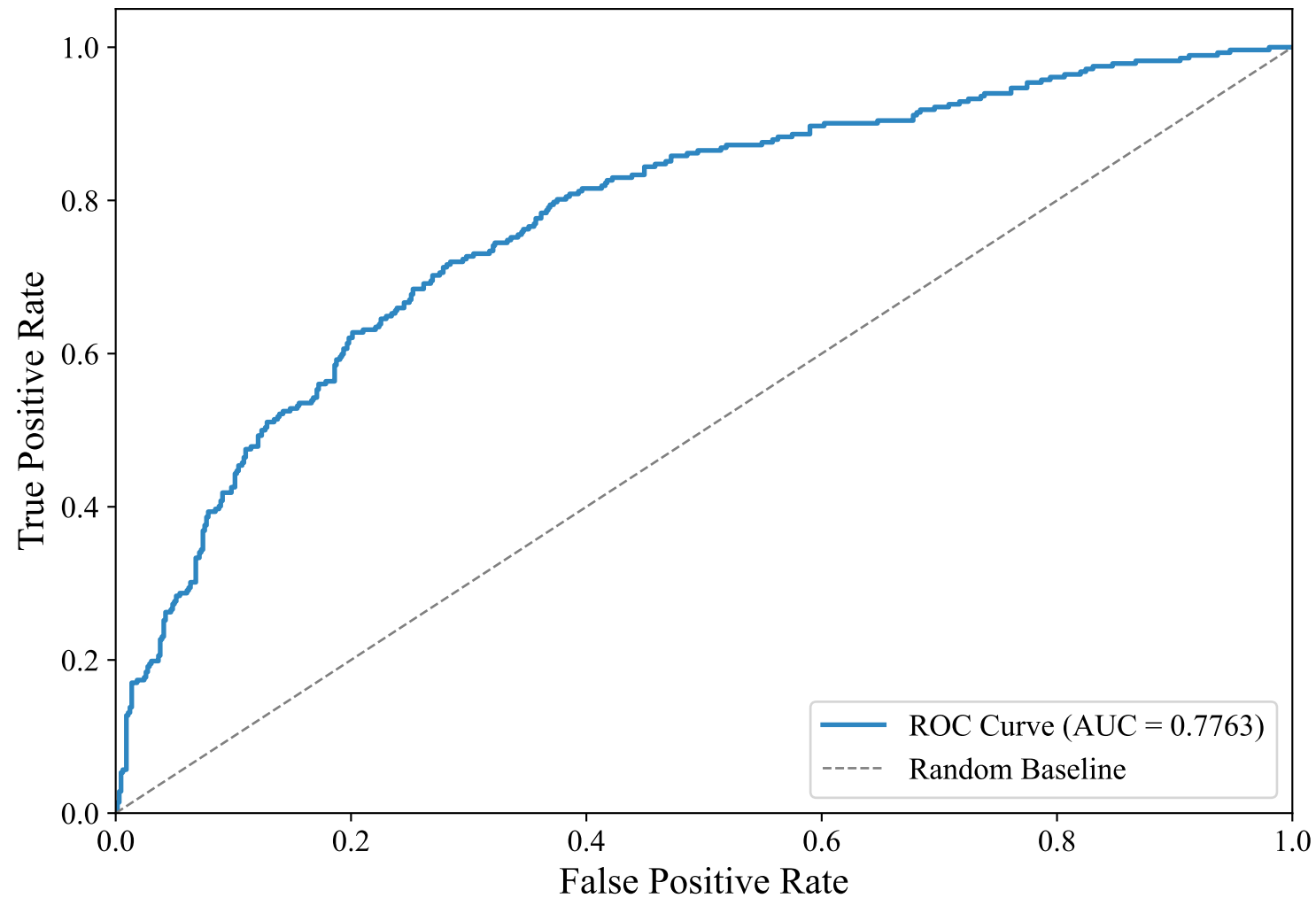
ROC Curve — ENGLISH_MANUAL (xlm-roberta-base, random_forest)
