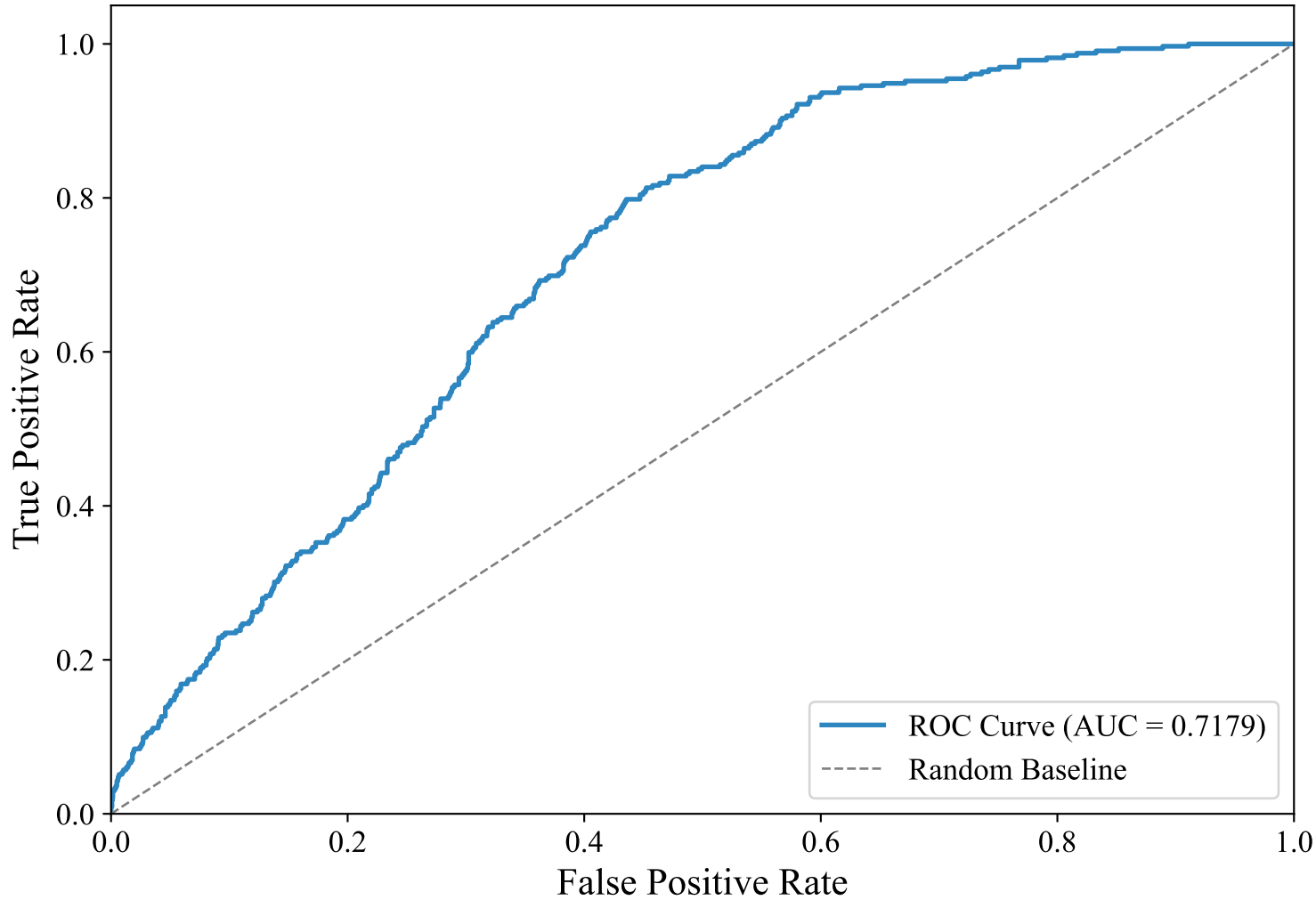
ROC Curve — GERMAN_MANUAL (multilingual-e5-large-instruct, svm_rbf)
