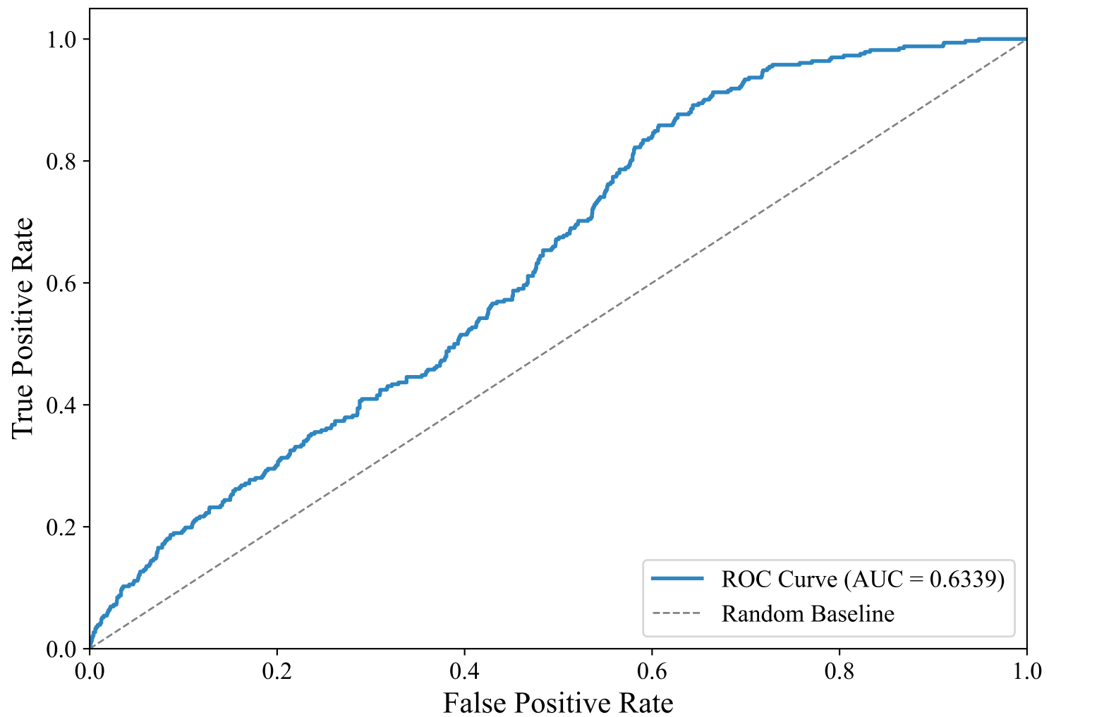
ROC Curve — GERMAN_MANUAL (multilingual-e5-large-instruct, xgboost)
