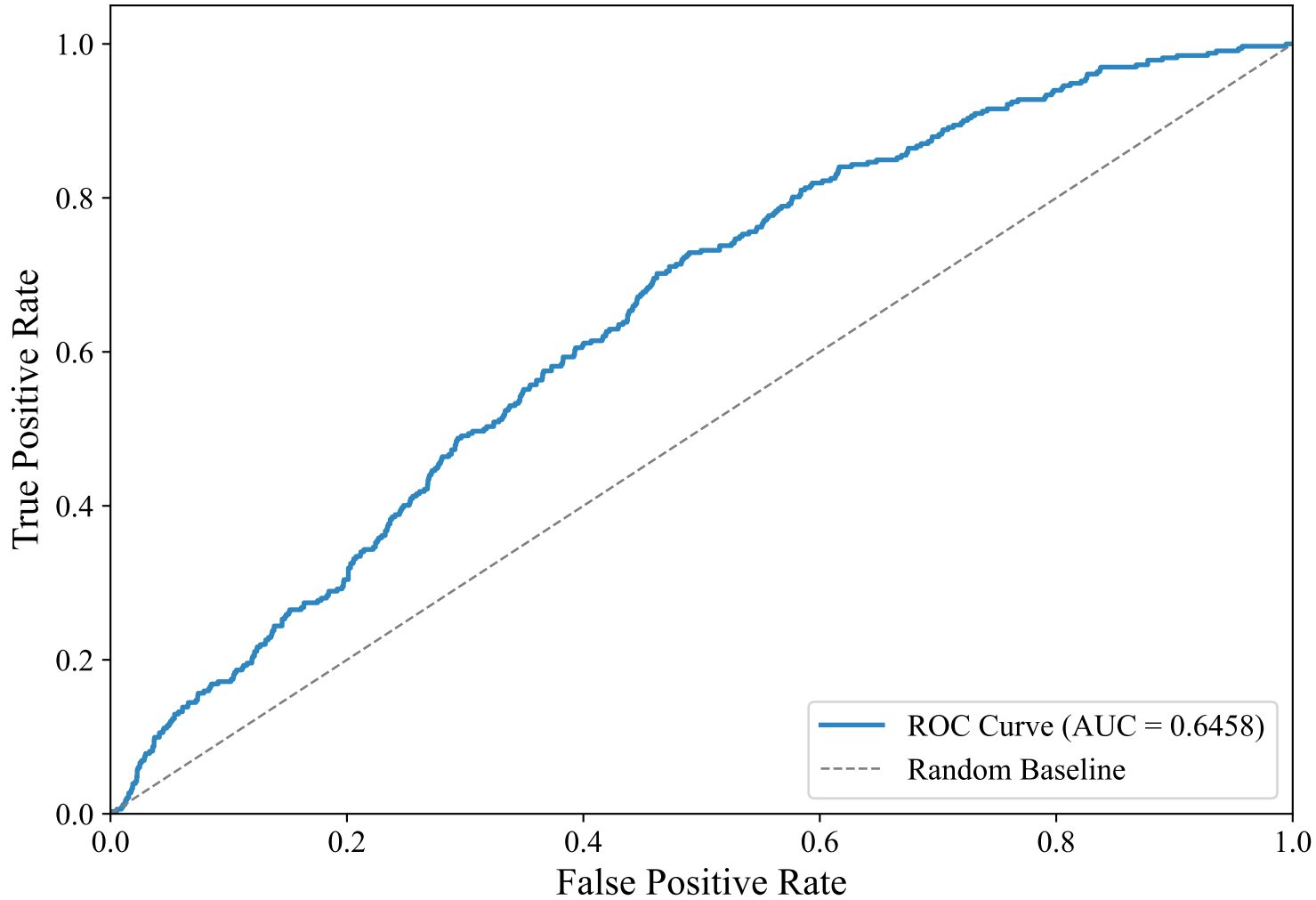
ROC Curve — GERMAN_MANUAL (paraphrase-multilingual-MiniLM-L12-v2, lightgbm)
