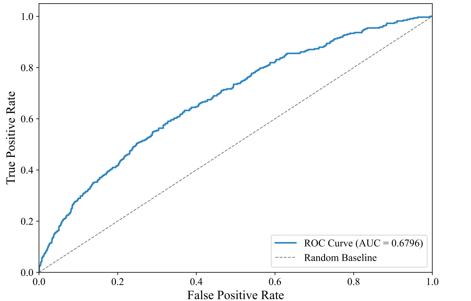
ROC Curve — GERMAN_MANUAL (paraphrase-multilingual-MiniLM-L12-v2, random_forest)
