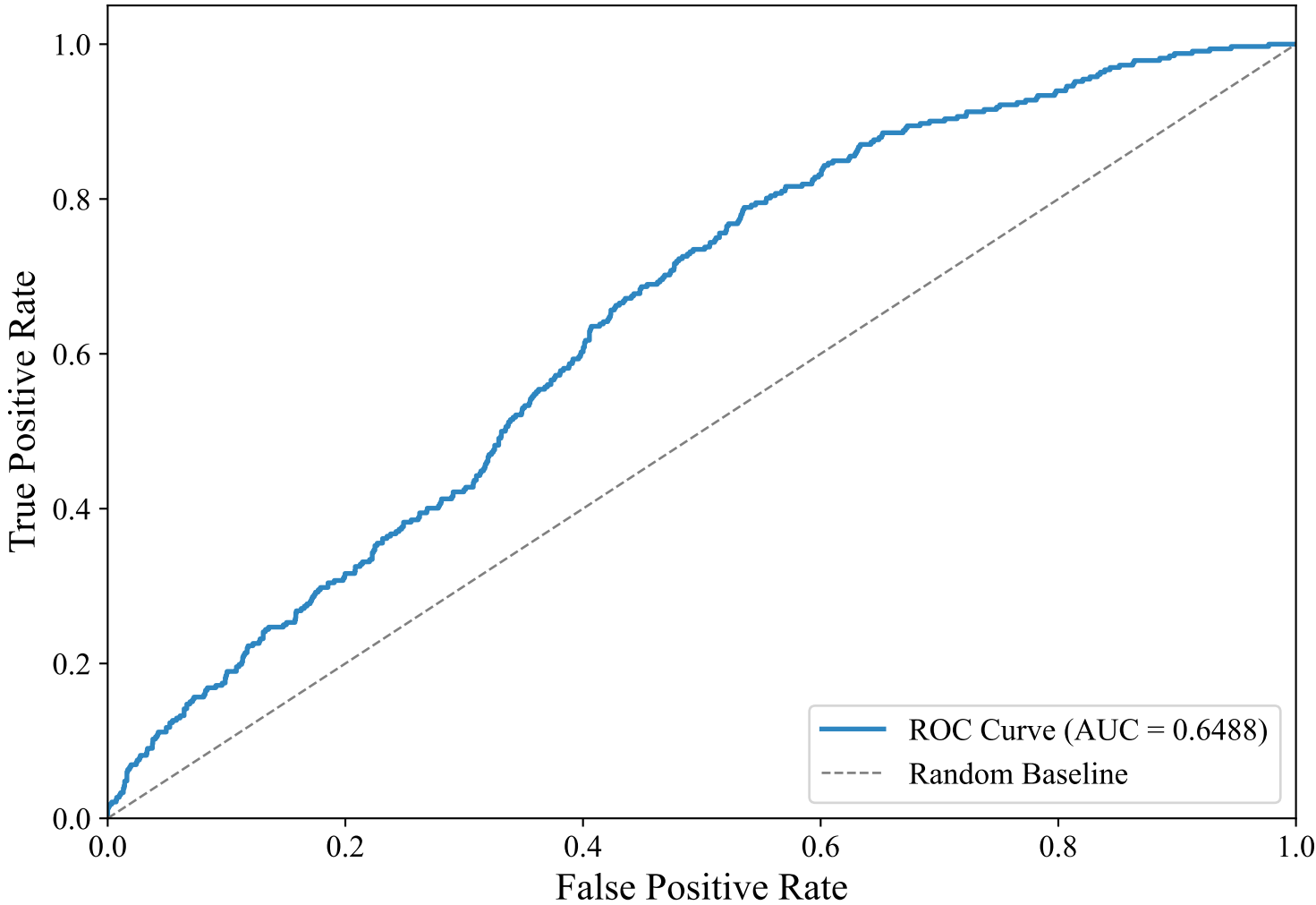
ROC Curve — GERMAN_MANUAL (paraphrase-multilingual-MiniLM-L12-v2, svm_linear)
