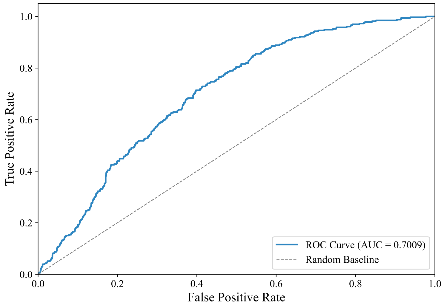
ROC Curve — GERMAN_MANUAL (paraphrase-multilingual-MiniLM-L12-v2, svm_rbf)
