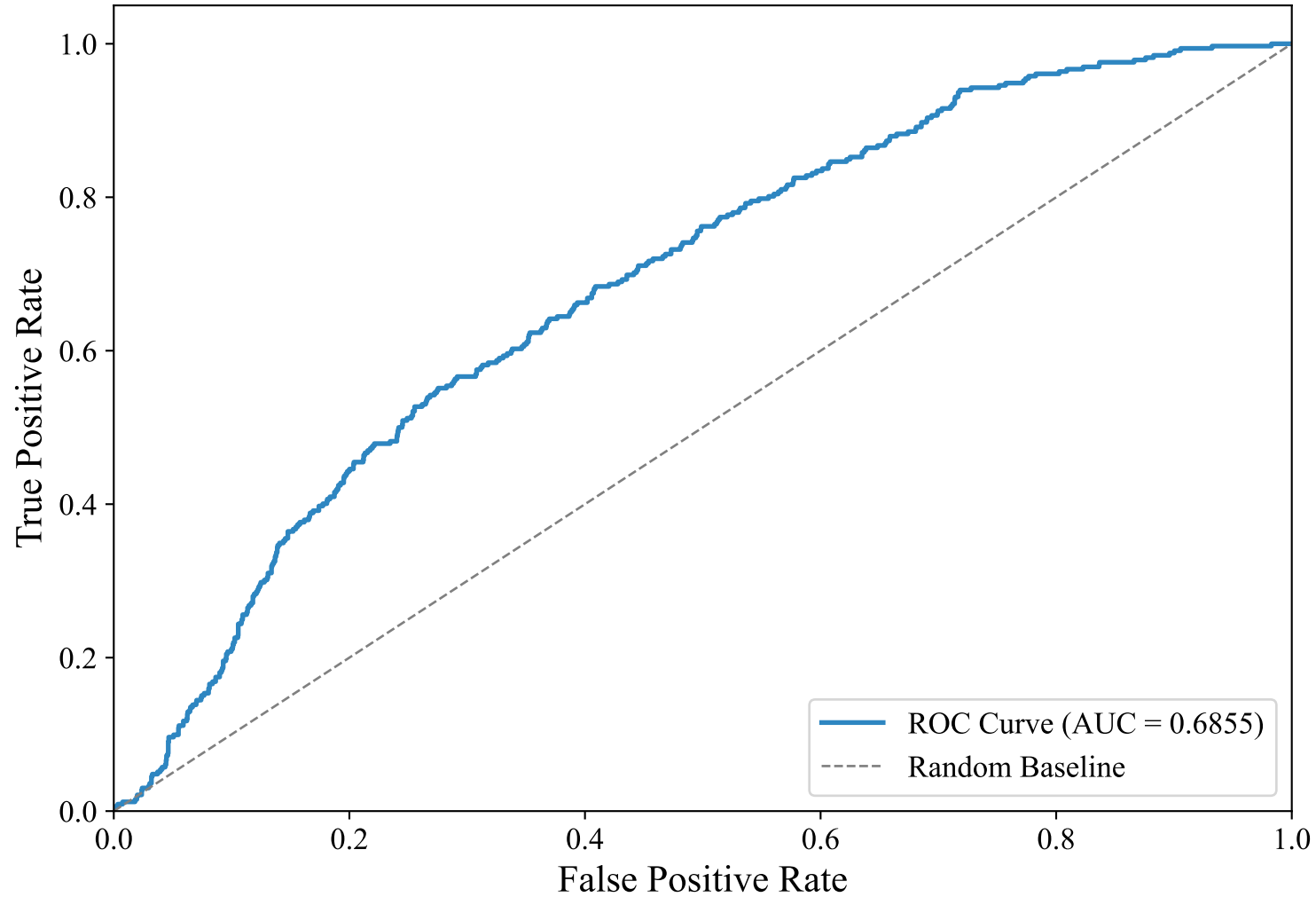
ROC Curve — GERMAN_MANUAL (paraphrase-multilingual-mpnet-base-v2, random_forest)
