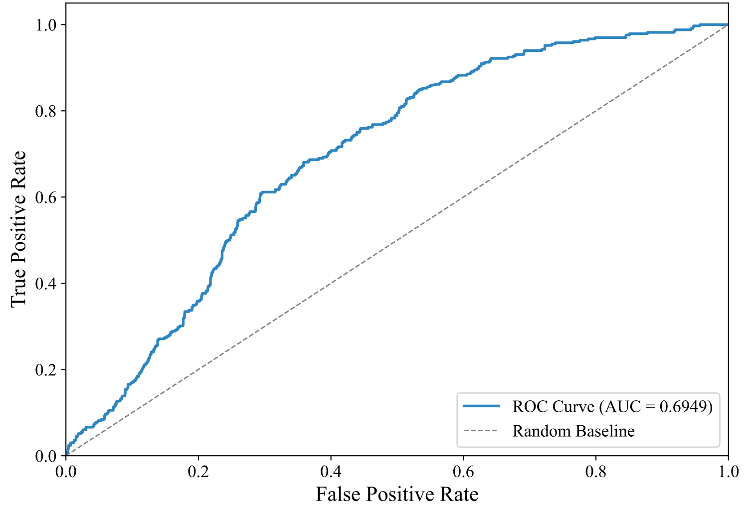
ROC Curve — GERMAN_MANUAL (paraphrase-multilingual-mpnet-base-v2, svm_rbf)
