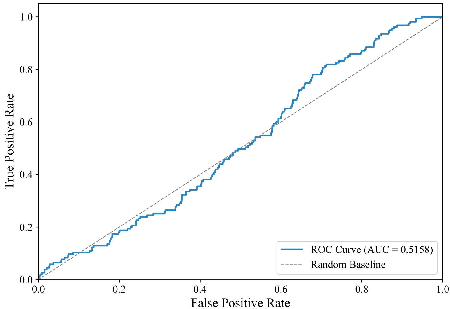
ROC Curve — SWEDISH_MANUAL (multilingual-e5-large-instruct, lightgbm)
