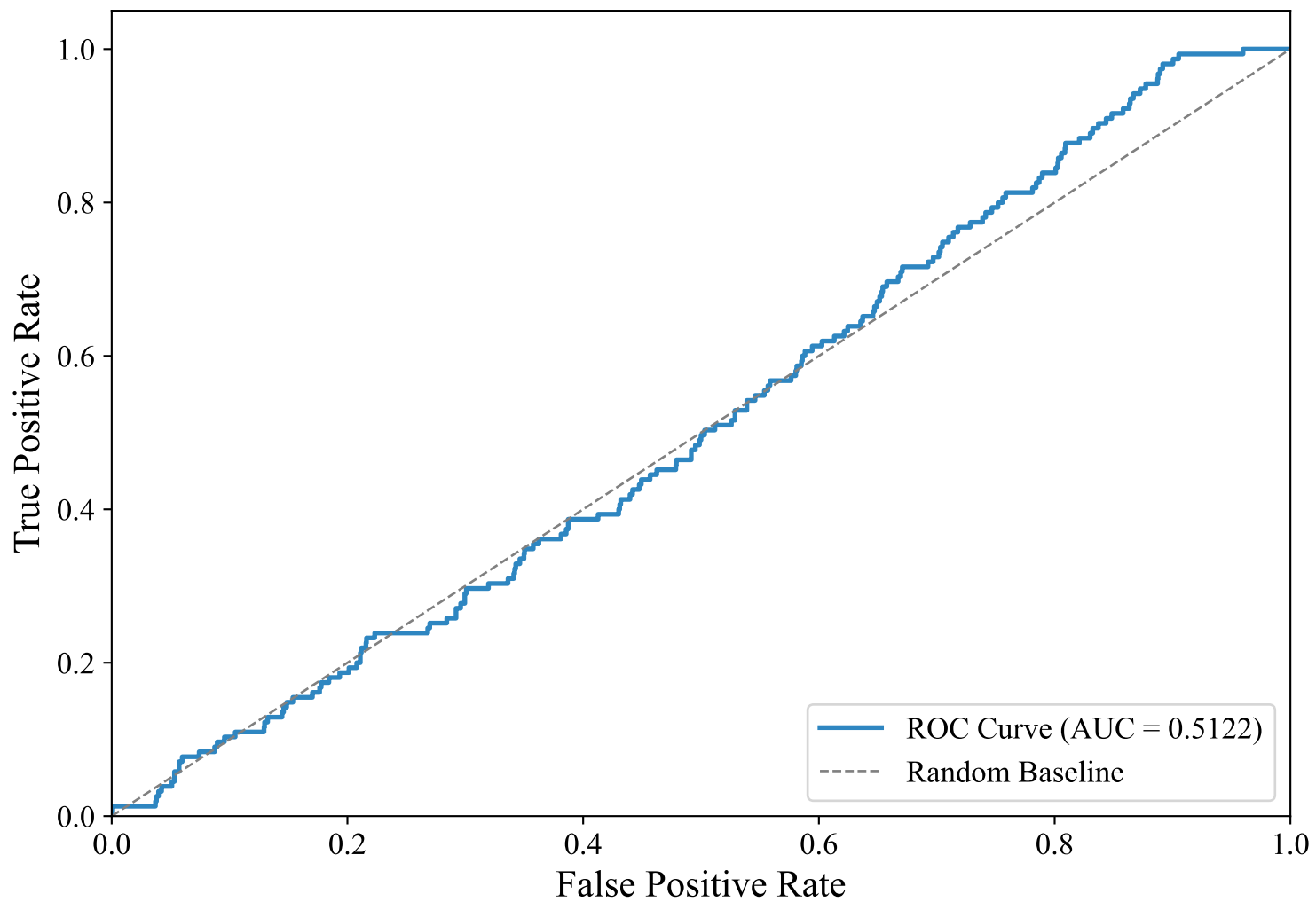
ROC Curve — SWEDISH_MANUAL (paraphrase-multilingual-MiniLM-L12-v2, lightgbm)
