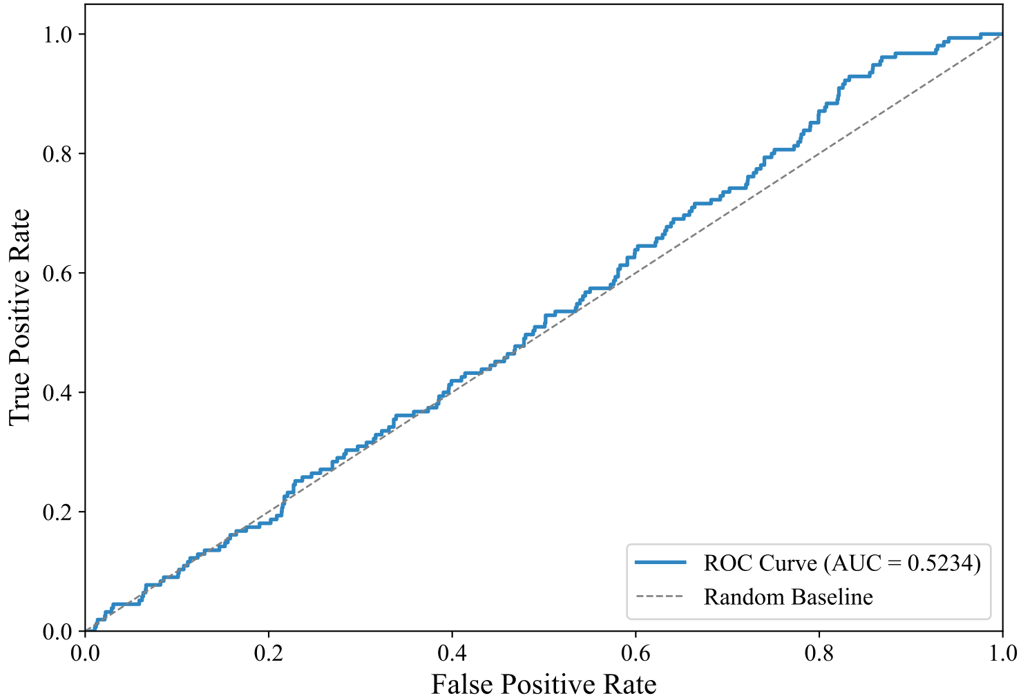
ROC Curve — SWEDISH_MANUAL (paraphrase-multilingual-MiniLM-L12-v2, random_forest)
