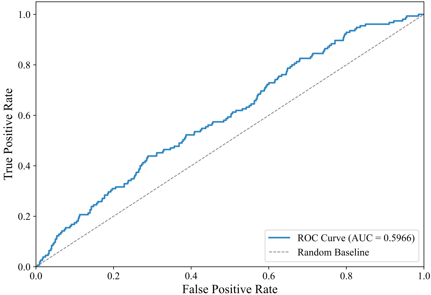
ROC Curve — SWEDISH_MANUAL (paraphrase-multilingual-MiniLM-L12-v2, svm_linear)
