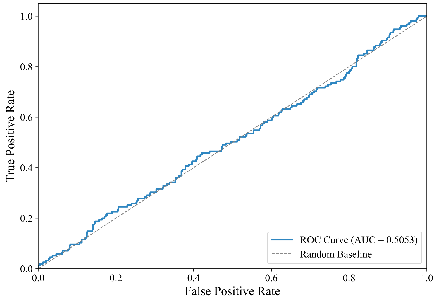
ROC Curve — SWEDISH_MANUAL (paraphrase-multilingual-mpnet-base-v2, lightgbm)
