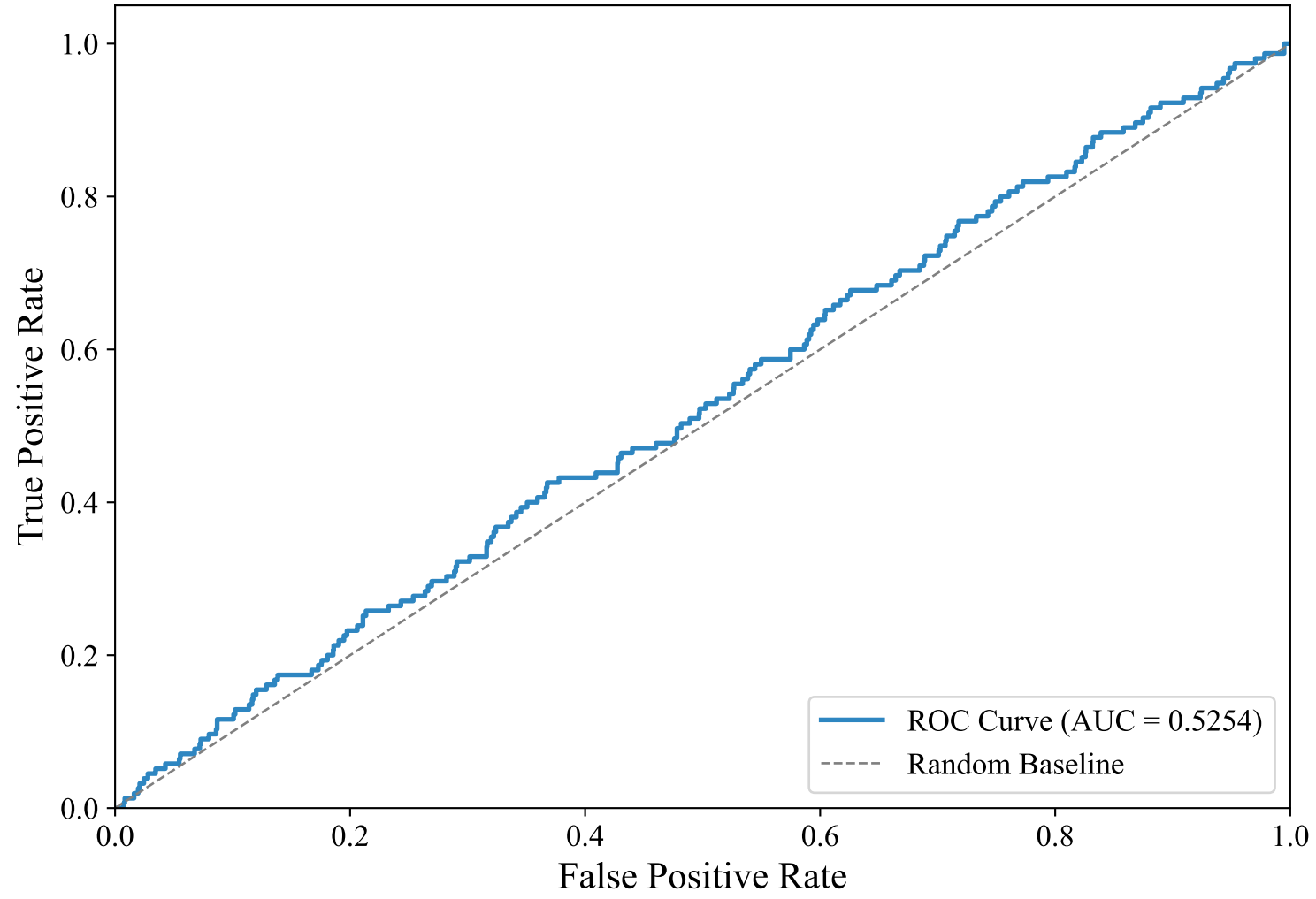
ROC Curve — SWEDISH_MANUAL (paraphrase-multilingual-mpnet-base-v2, random_forest)
