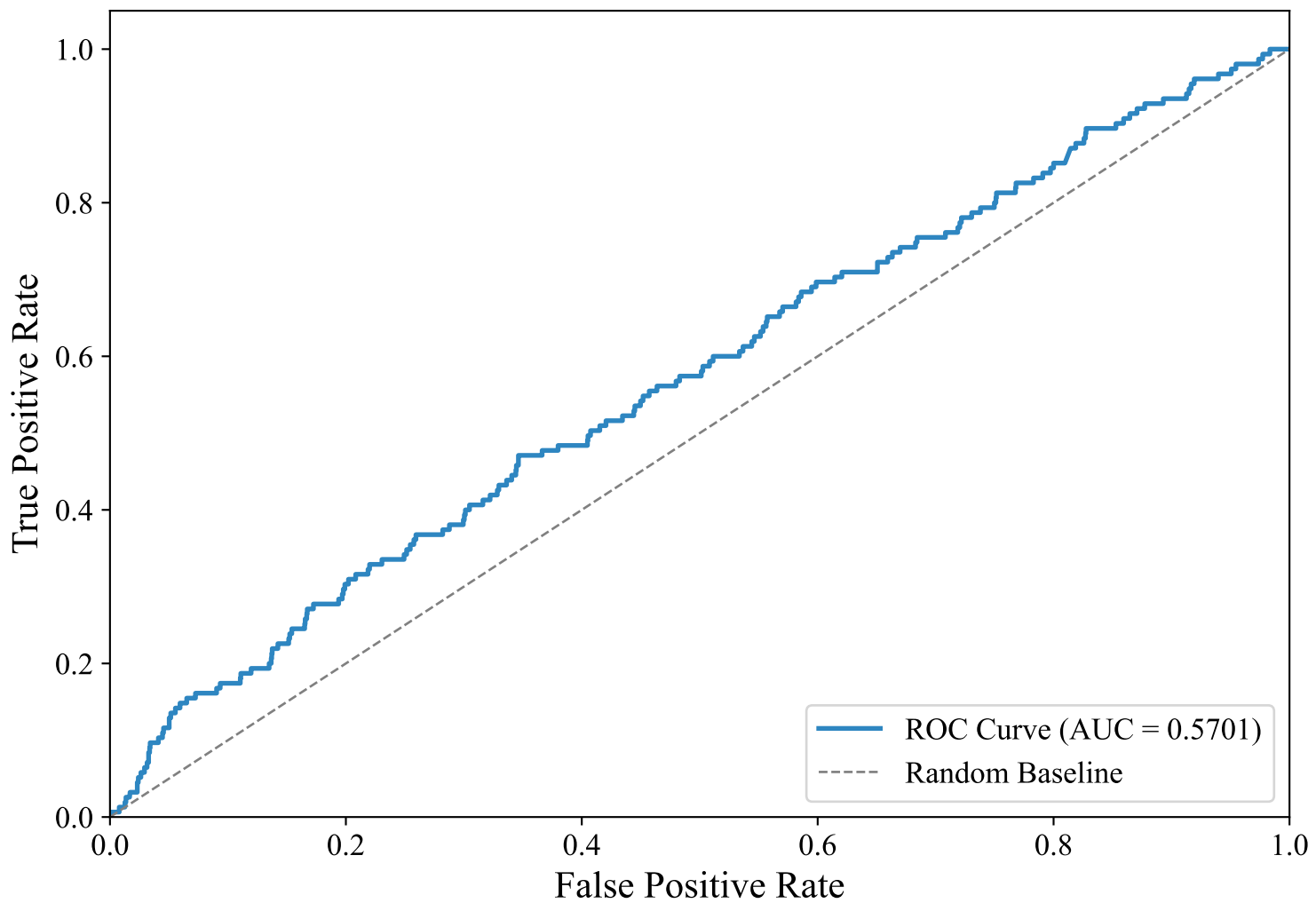
ROC Curve — SWEDISH_MANUAL (paraphrase-multilingual-mpnet-base-v2, svm_rbf)
