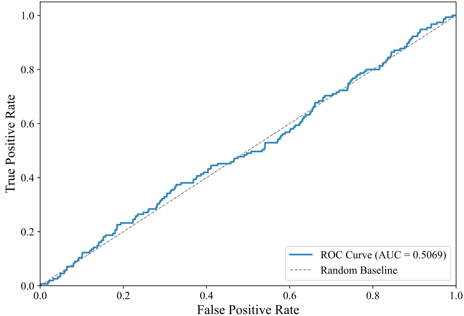
ROC Curve — SWEDISH_MANUAL (paraphrase-multilingual-mpnet-base-v2, xgboost)
