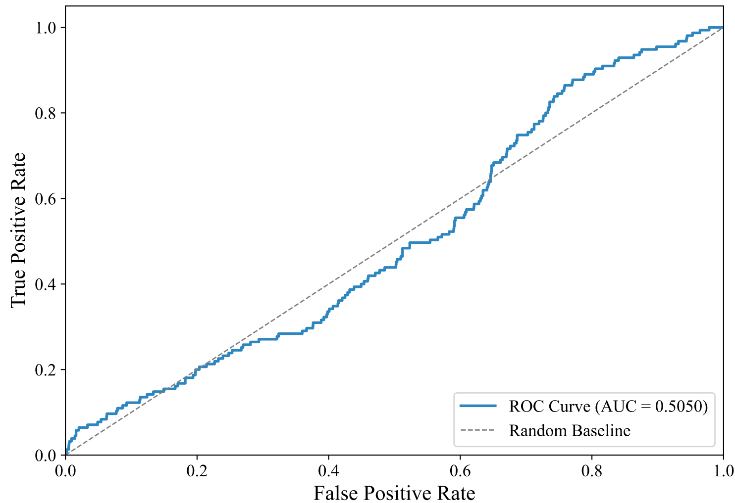
ROC Curve — SWEDISH_MANUAL (snowflake-arctic-embed-l-v2.0, random_forest)
