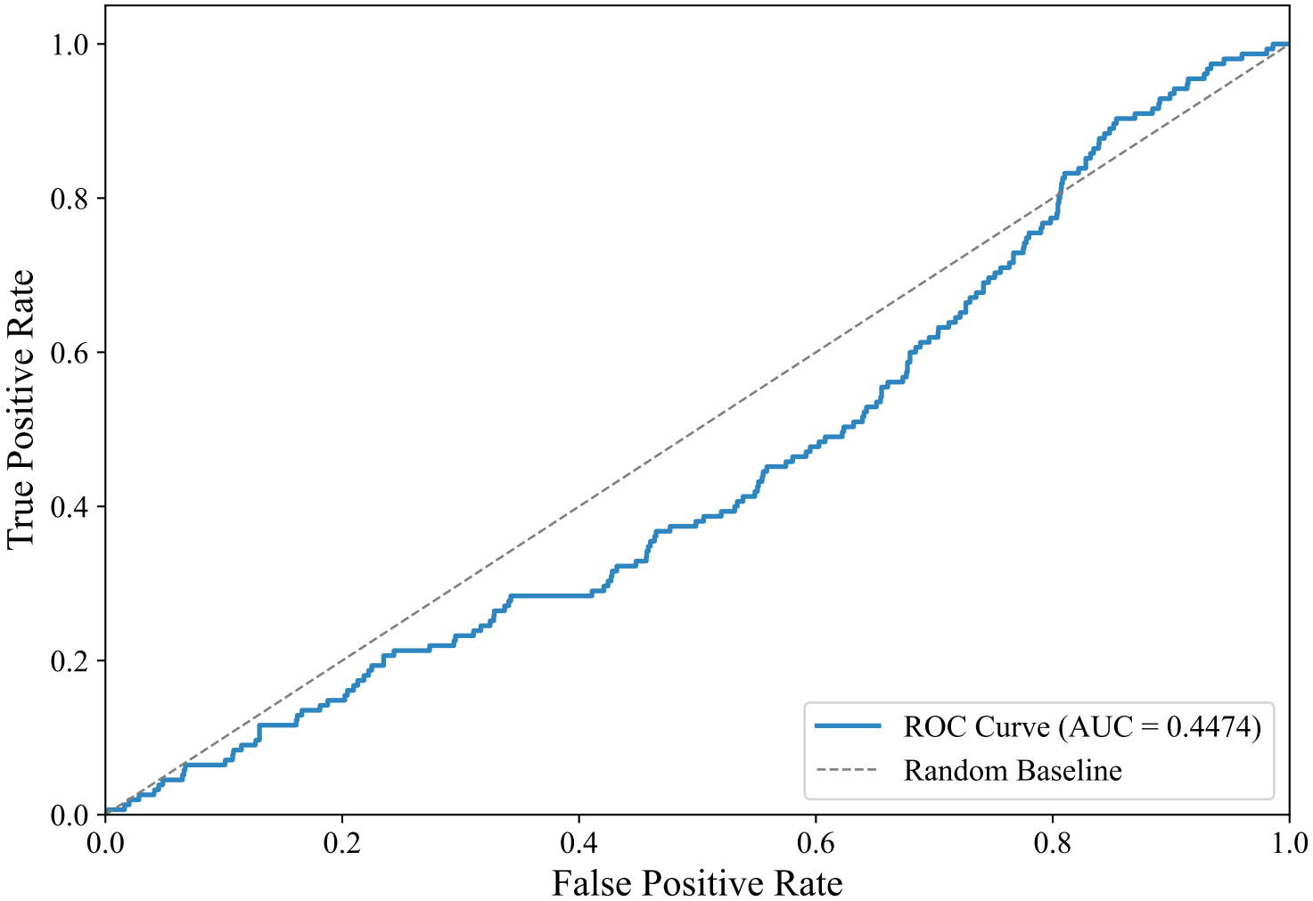
ROC Curve — SWEDISH_MANUAL (snowflake-arctic-embed-l-v2.0, xgboost)
