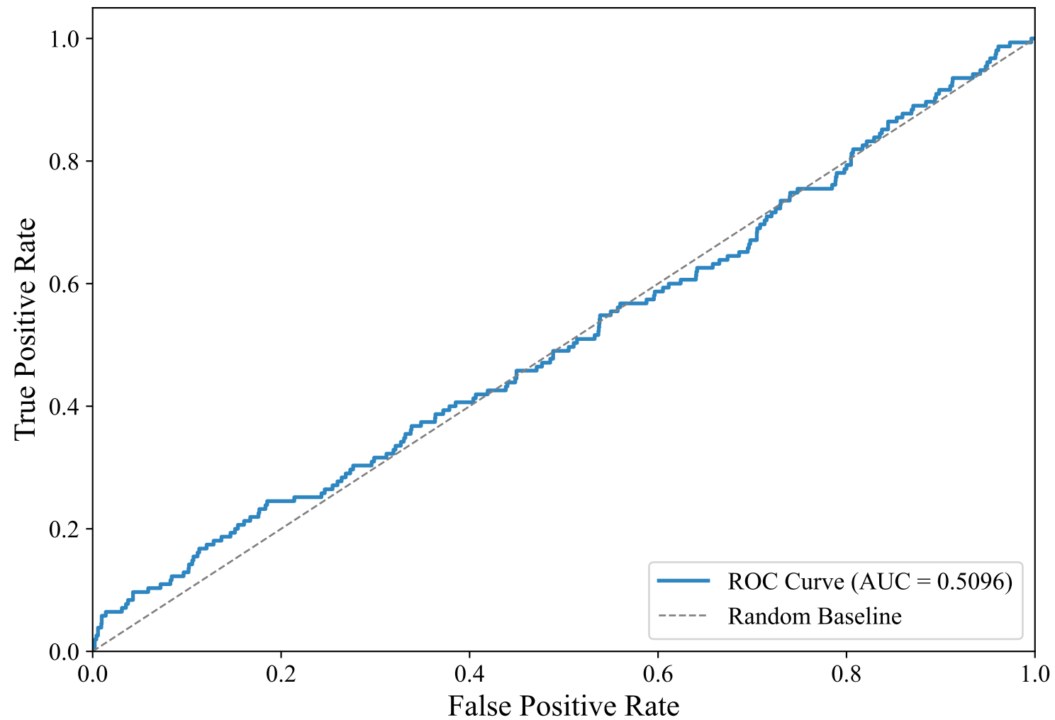
ROC Curve — SWEDISH_MANUAL (xlm-roberta-base, svm_rbf)
