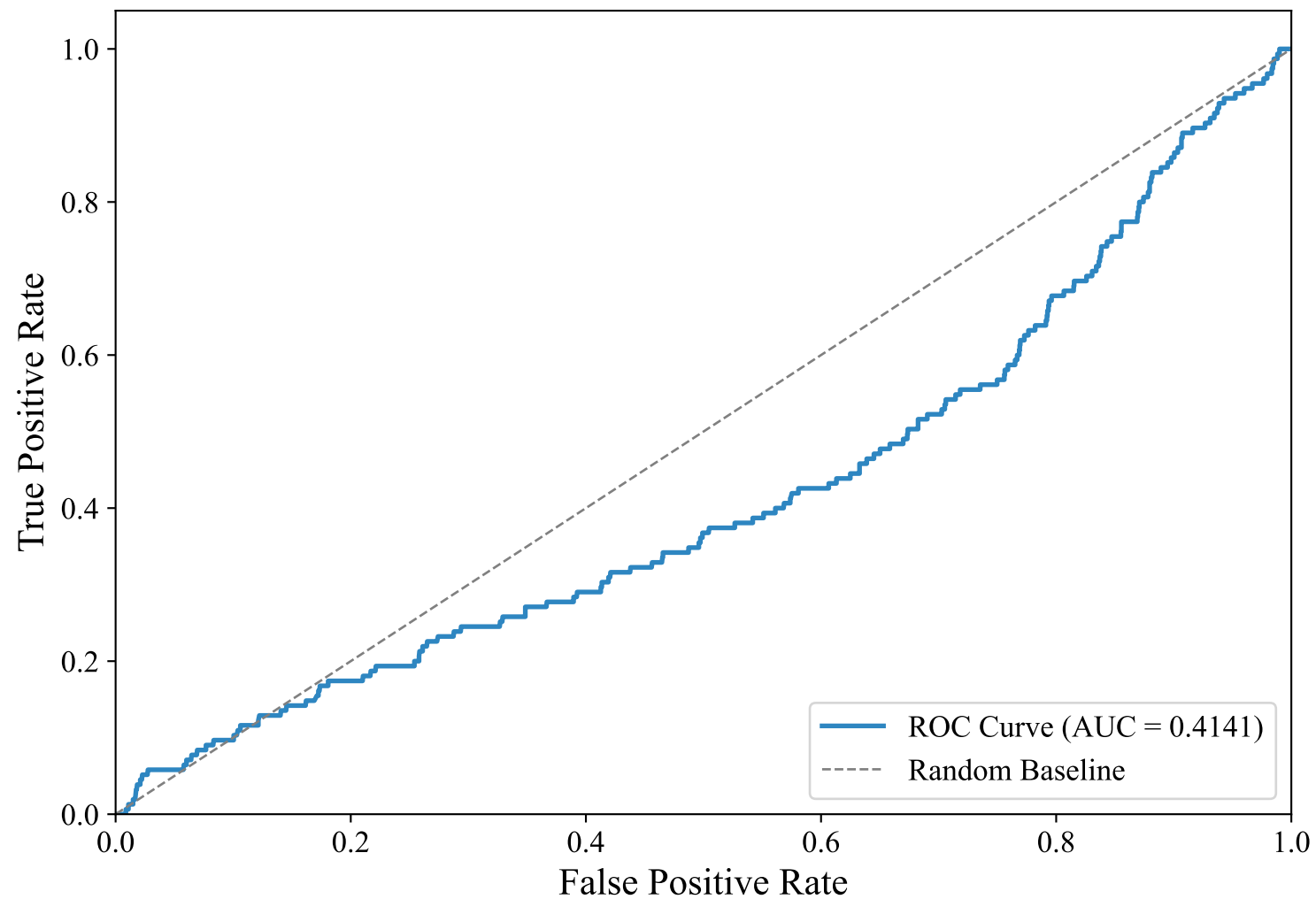
ROC Curve — SWEDISH_MANUAL (xlm-roberta-base, xgboost)
