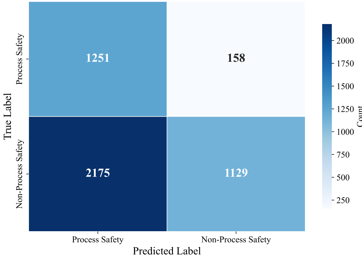
Confusion Matrix — English (XLM-RoBERTa XNLI, Zero-Shot)
